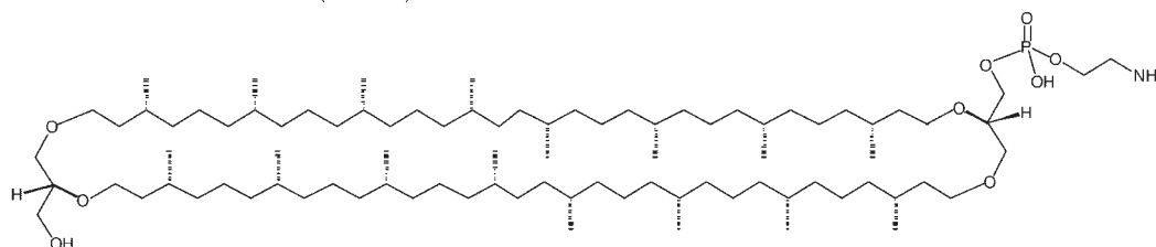
(r) Di-glycerol tetraether phospholipids (cardarchaeols): sn -cardarchaeo-1-phosphoethanolamine
