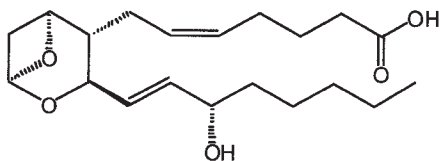
(r) Thromboxanes: Thromboxane A2; 9S,11S-epoxy,15S-hydroxy-thromboxane-5Z,13E-dien-1-oic acid
