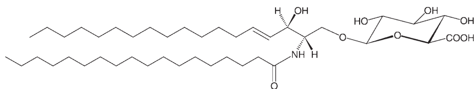
(n) Acidic Glycosphingolipids: Glucuronosphingolipids: GlcUAβ-Cer(d18:1/18:0)
