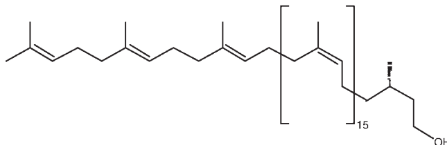
(k) Dolichols: Dol-19; α-dihydrononadecaprenol
