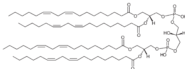
(n) Diacylglycerophosphoglycerophosphodiradylglycerols: 1',3'-Bis[1,2-di-(9Z-12Z-octadecadienoyl)- sn -glycero-3-phospho]- sn -glycerol
