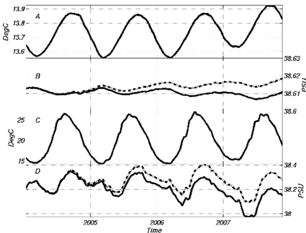
Fig. 2. (A) Time series of mean volume temperature. Solid (MFS_V2.1) and dashed (MFS_V2.2) lines overlap. (B) Time series of mean volume salinity, solid line indicates MFS_V2.1 results, dashed line indicates MFS_V2.2 results. (C) Time series of mean surface temperature, solid line (MFS_V2.1) and dashed (MFS_V2.2) lines overlap. (D) Time series of mean surface salinity, solid line indicates MFS_V2.1 results, dashed line indicated MFS_V2.2 results.
