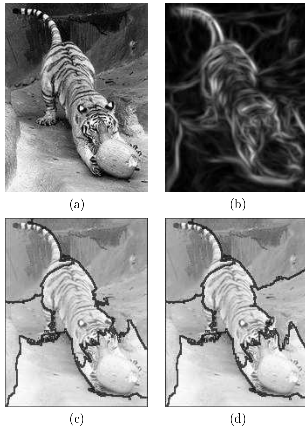
Figure 2: Image segmentation by the MNCut algorithm: (a) the original image; (b) the output of the edge detector; (c,d) segmentation by MNCut using the first 6 respectively 7 eigenvectors and k-means clustering. Two pixels are dissimilar if they are more than 30 apart or if they are separated by an edge; otherwise they are considered similar. Note that even with this simple similarity measure and in spite of the many stripes, most of the tiger is segmented correctly.
