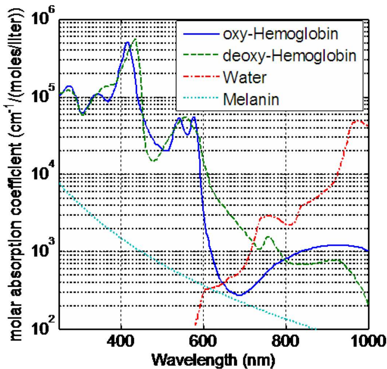
Figure 3. Molar absorption coefficients of common absorbers in tissue: oxy-hemoglobin, deoxy-hemoglobin, melanin, and water.
