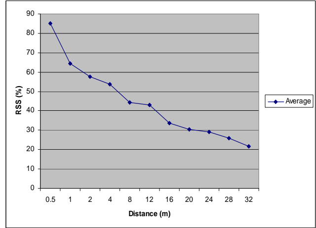
Figure 7 Averaging RSS values (see online version for colours)
