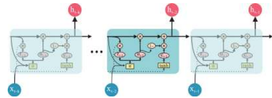
FIGURE 6. The architecture of the GRU model.
