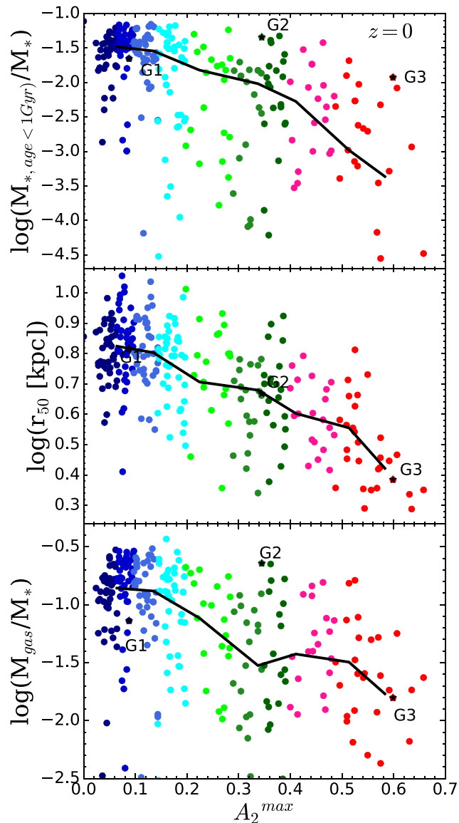
Figure 5. Bar strength parameter A_2^{\max} as a function of gas mass fraction (bottom), of half-mass radius (middle) and of the stellar mass form in the last Gyr at z = 0 for all discs in our sample. Solid lines trace the median as a function of bar strength. G1, G2 and G3 refer to galaxies 1, 2 and 3 in Fig. 2, respectively.
