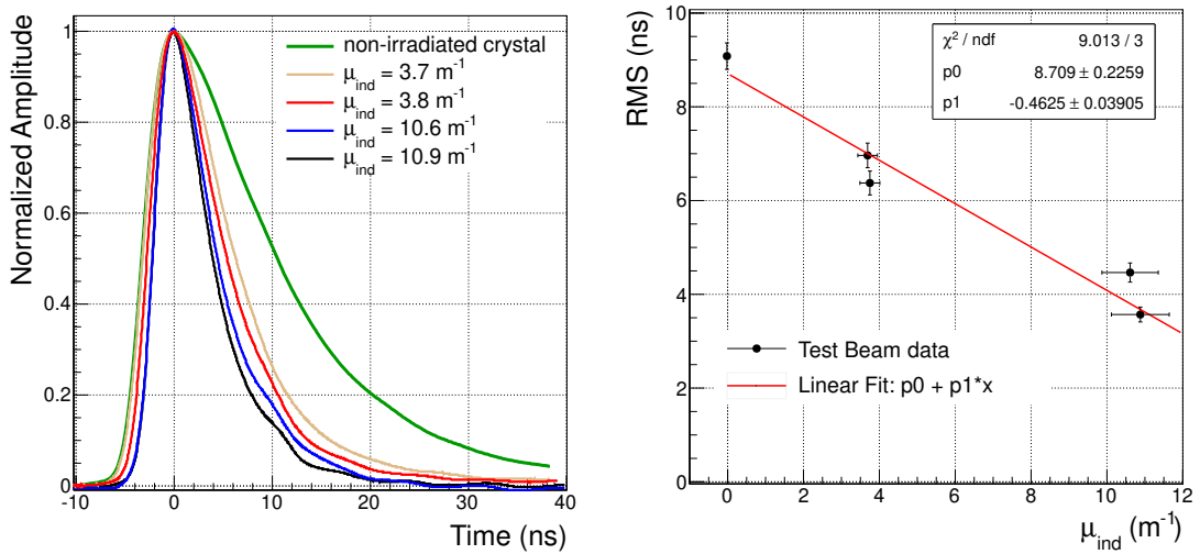
Figure 19. Left: waveforms of a non-irradiated crystal and four proton-irradiated crystals are shown. The \mu_{\text{ind}} of the irradiated crystals varies between 3.7 \text{m}^{-1} and 10.9 \text{m}^{-1} . Right: correlation between \mu_{\text{ind}} and RMS of the average pulse fitted with a linear function (red).
