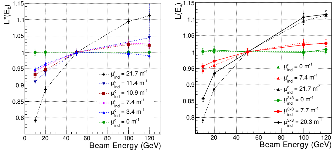
Figure 17. Left: linearity curves for central crystal only. Right: comparison of linearity for 3 \times 3 clusters with the linearity of the corresponding central crystals for 2012 matrices 3 and 4.
