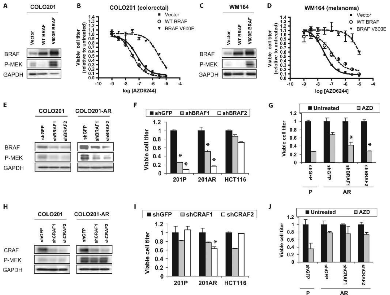
Fig. 3. Increased BRAF V600E is responsible for AZD6244 resistance in AR cells. ( A and C ) Western blots of COLO201 ( A ) and WM164 ( C ) cells infected with retroviruses encoding wild-type (WT) BRAF, mutant V600E BRAF, or vector control. ( B and D ) COLO201 ( B ) or WM164 ( D ) cells expressing WT BRAF, V600E BRAF, or vector control were treated with the indicated concentrations of AZD6244 for 72 hours and viable cell titer was determined. ( E and H ) Western blots of COLO201 and COLO201-AR cells infected with control shRNA (shGFP) or two different shRNAs directed against either BRAF ( E ) or CRAF ( H ). After infection, cells were selected in puromycin for 96 hours. Experiments were performed at least three times. ( F and I ) COLO201 (201P), COLO201-AR (201AR), and the KRAS mutant HCT116 cell line were infected with the above shRNAs. Cell viability was determined after 5 days of puromycin selection. Viral titers were used that yielded about the same results in the presence or absence of puromycin. *P < 0.001 relative to HCT116 cells infected with corresponding shRNA. ( G and J ) COLO201 (P) and COLO201-AR (AR) cells infected with the indicated shRNAs were selected in puromycin for 48 hours and then treated with or without 100 nM AZD6244 (AZD) for 72 hours before determination of cell viability. Viable cell titer is shown relative to the untreated control for each shRNA. *P < 0.001 relative to shGFP-infected COLO201-AR cells treated with AZD6244.
