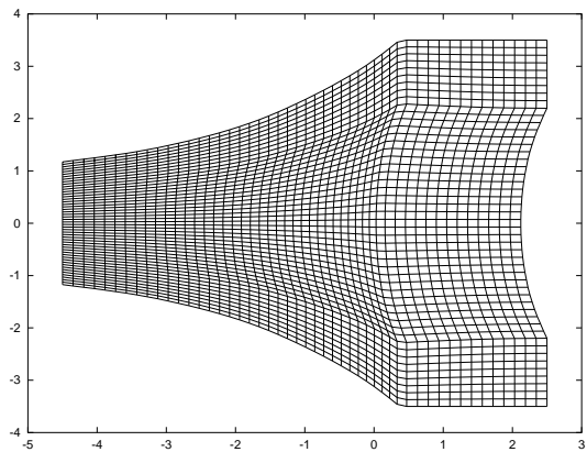
Figure 6. Contour mesh.
