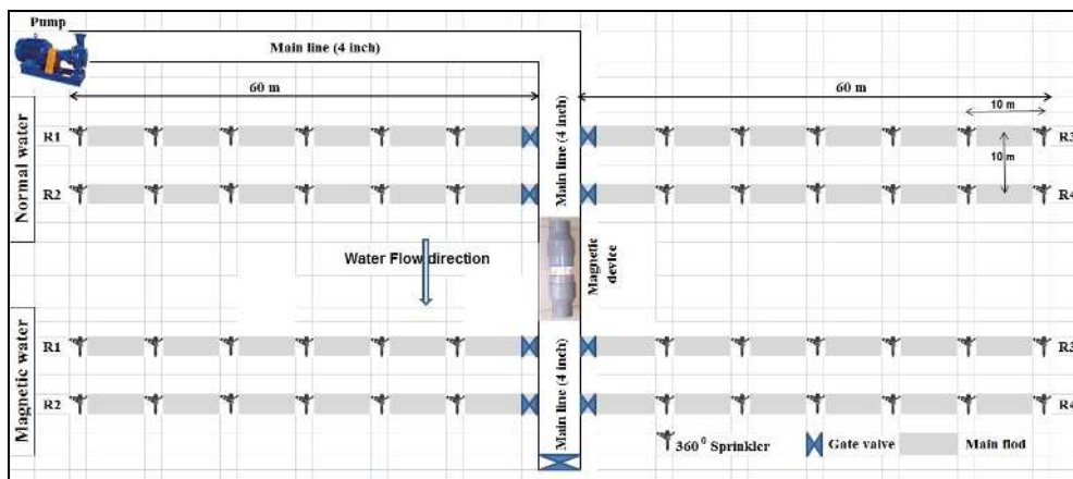
Fig. (1): Layout of experiment design under solid set sprinkler system.
