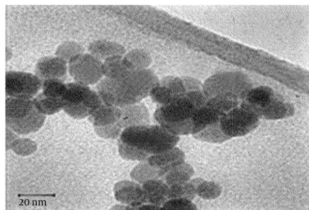
Figure 2. Transmission Electron Microscopy Image of Zinc Oxide Nanoparticles
