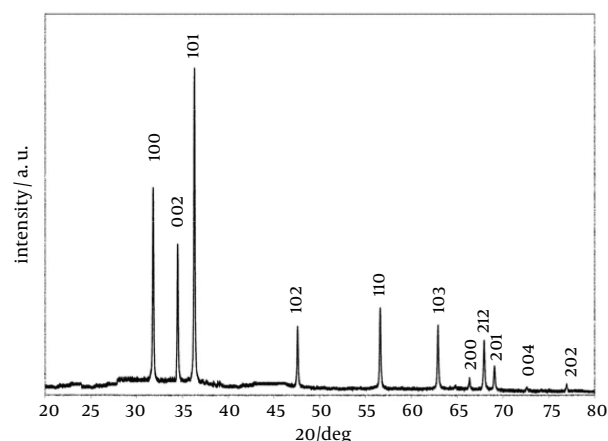
Figure 1. Powder X-ray Diffraction Pattern of Zinc Oxide Nanoparticles
