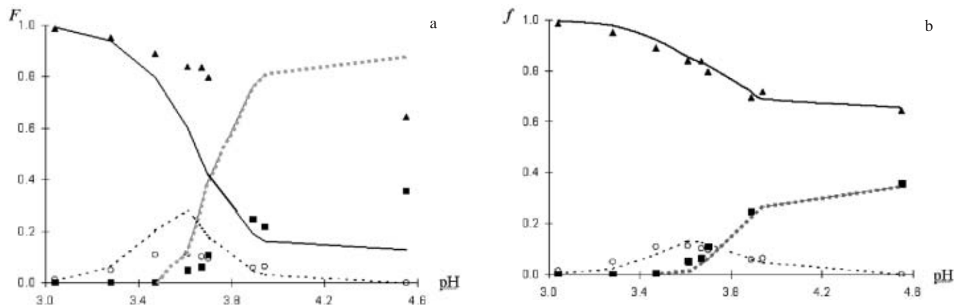
Fig. 3. Comparison of fractions determined with the model calculated by SUPERQUAD and area fractions obtained by 27 Al-NMR. ▲ 0ppm, ○ 5 ppm, and ■ 63 ppm experimental fractions. — monomers, - - - trimer, and -·-·- tridecamer estimated fractions. (a) Component fractions. (b) Species fractions: It should be noticed that the fit is accomplished, practically, over the corresponding species distribution diagram.
