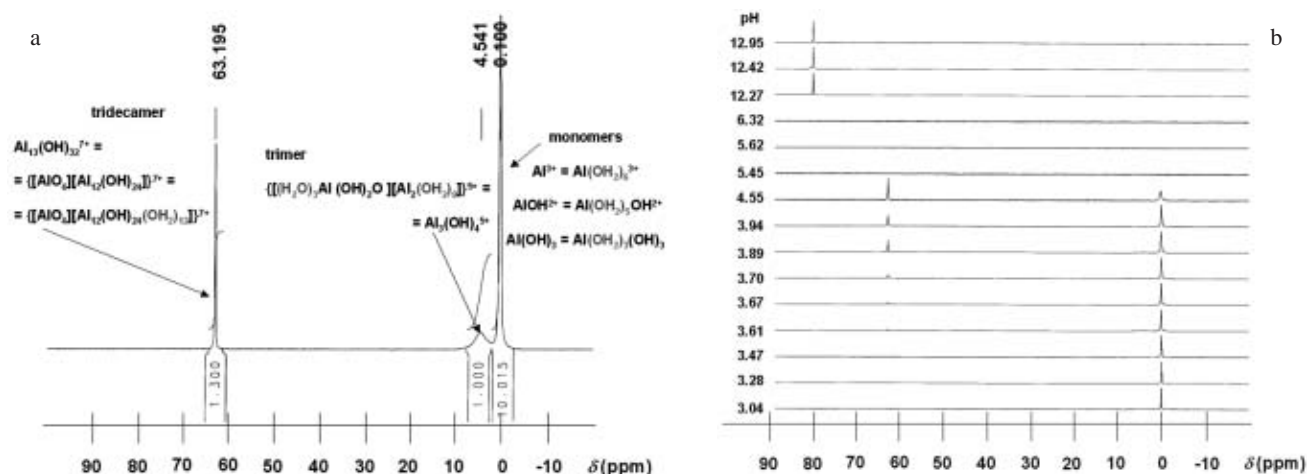
Fig. 2. Typical ^{27}\text{Al} -NMR spectra for Al(III)-H 2 O system with [\text{Al(III)}]_{\text{total}} = 0.500 M. (a) Spectrum for a pH = 3.89 showing chemical shifts, integration of signals and species assigned to each signal (see text for explanation of these assignments). (b) Variation of NMR spectrum with pH. It should be noticed the inversion of area ratio ( A_{\text{tridecamer}}/A_{\text{monomers}} , from a value less than unit to another greater than unit) for 63 ppm and 0 ppm signals, when pH changes from 3.94 to 4.55. Also, it is remarkable the great broadening and weakening for the 0 ppm signal at the same pH values.
