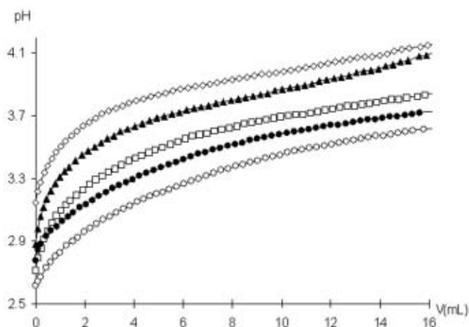
Fig. 1. Typical potentiometric titrations, with standardized NaOH, of Al(III)-H 2 O system for different [Al(III)] total values: \diamond 0.100 M, \blacktriangle 0.200 M, \square 0.300 M, \bullet 0.400 M, \circ 0.500 M.
