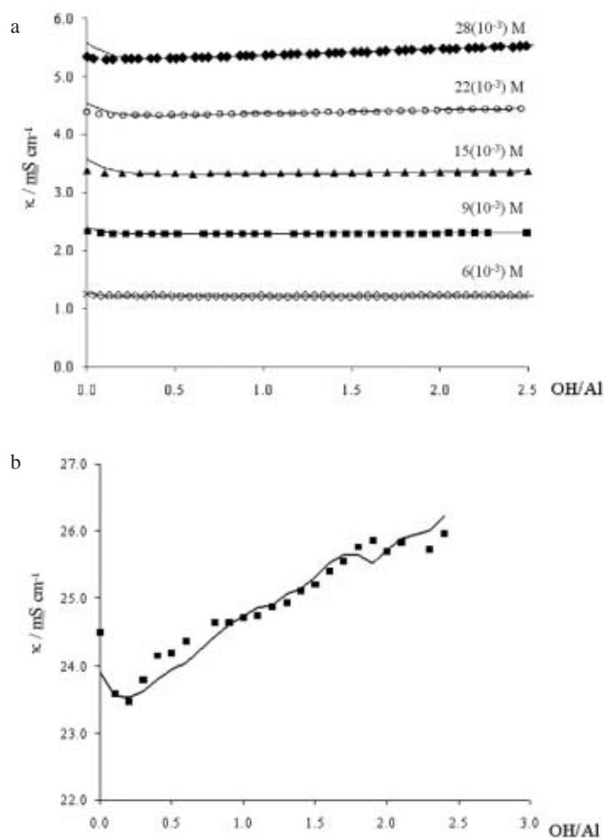
Fig. 4. Conductometric titrations curves for the Al(III)-H 2 O system with different [Al(III)] total values. The solid lines represent the conductivity estimated using the model obtained by means of the SUPERQUAD program. The markers represent the experimental conductivity values. (a) 6.00(10^{-3})\text{M} \leq [\text{Al(III)}]_{\text{total}} \leq 28.0(10^{-3})\text{M} . (b). [\text{Al(III)}]_{\text{total}} = 0.12\text{M} .
