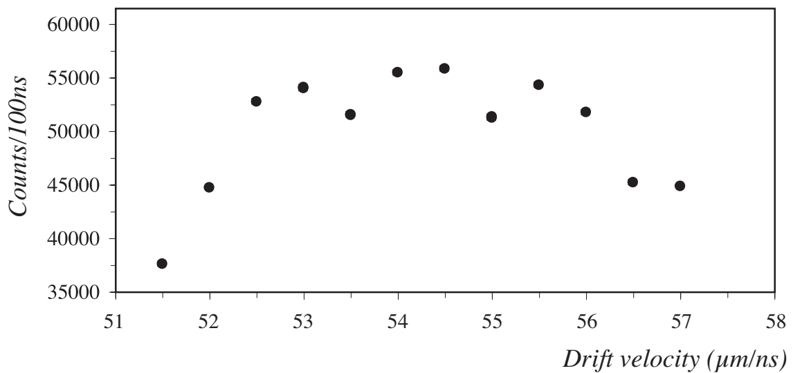
Figure 8- Autotrigger rate on a MB3 type chamber (HH and HL triggers only) for cosmoics as a function of the drift velocity settings. The regular efficiency drop every three steps is due to an hardware bug in the BTI ASIC which cannot be corrected. The hole is filled when allowing uncorrelated triggers.
