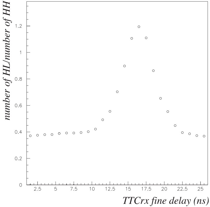
Figure 3- Ratio of HL to HH trigger type from external trigger data for a MB3 type chamber in 2003 beam test.
