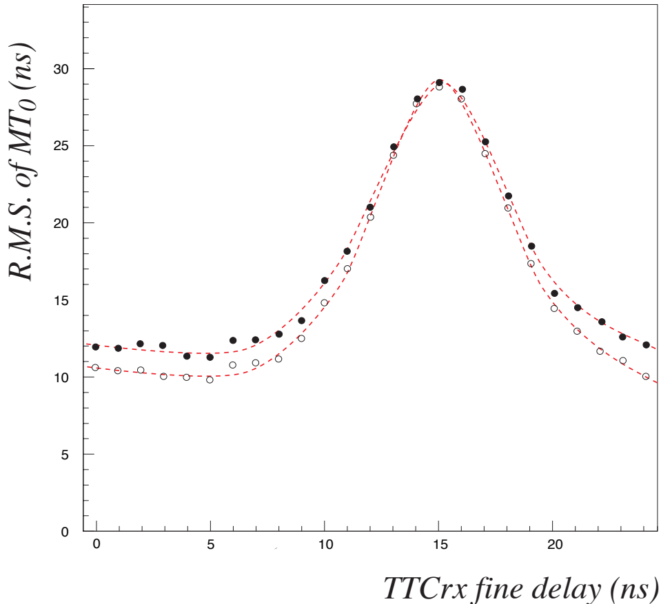
Figure 5- R.m.s. of MT_0 distribution for |MT_{01}-MT_{02}| < 1\sigma (open circles) and (b) |MT_{01}-MT_{02}| < 3\sigma (full circles). Data are for an MB3 chamber in 2003 beam test. Lines are drawn just to guide the eye.
