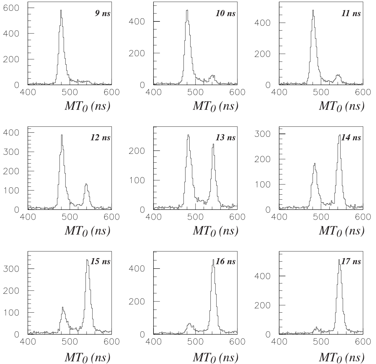
Figure 4- Evolution of the quantity MT_0 while increasing the fine delay of TTCrx. Plots are obtained for an MB3 type chamber during 2003 beam test.
