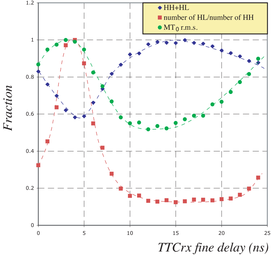
Figure 6- Behaviour as a function of the TTCrx delay of the trigger efficiency (HH+HL fraction), ratio of HL to HH and r.m.s. of MT 0 distribution. Data are for muons incident at 0° on a MB1 type chamber during 2004 beam test. Due to the large difference in absolute values of the three quantities, they are shown normalized to their highest value in order to allow better comparison among them. Lines are drawn to guide the eye.
