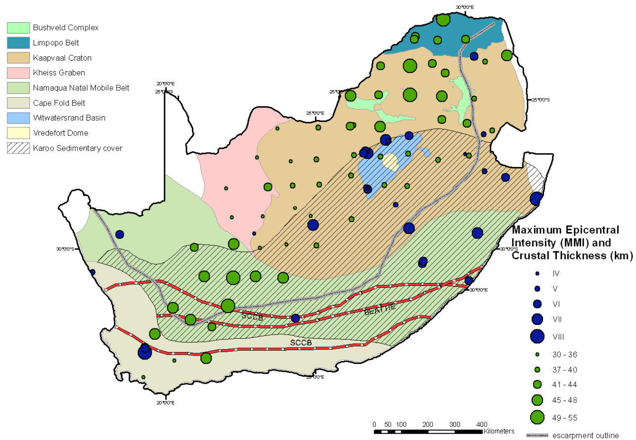
Figure 2 Geological provinces and crustal thickness results from Nguuri et al. (2001).
