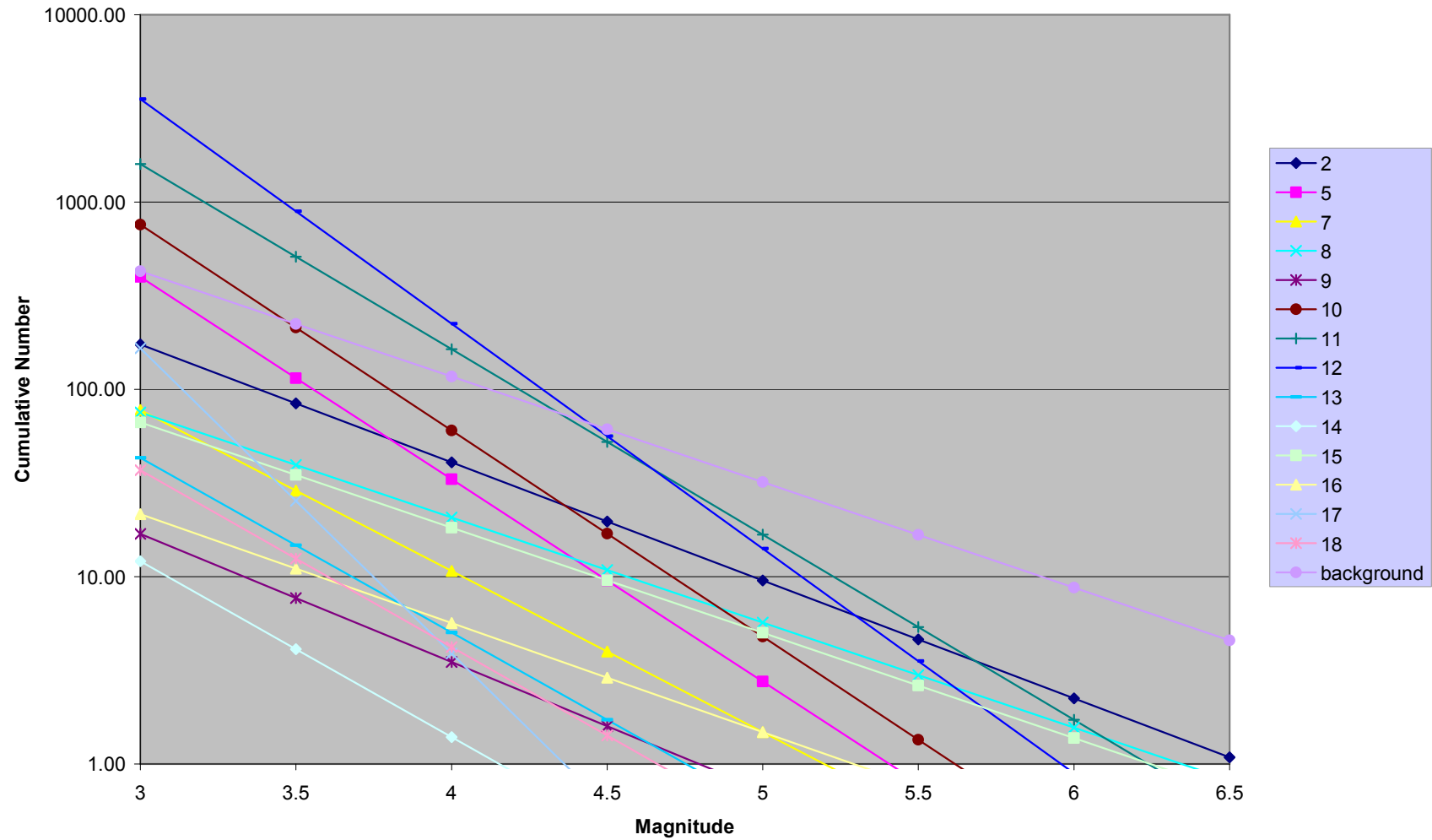
Figure 8 Plot of Gutenberg-Richter frequency magnitude relations for seismicity within each zone. Note that no solution could be obtained for Zones 1, 3, 4, 6 and 19 due to insufficient seismicity data within each zone
