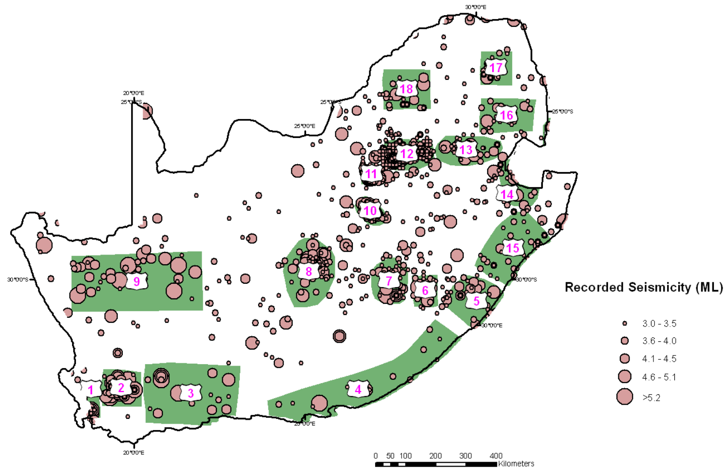
Figure 3 CEF schema consisting of 18 clusters.
