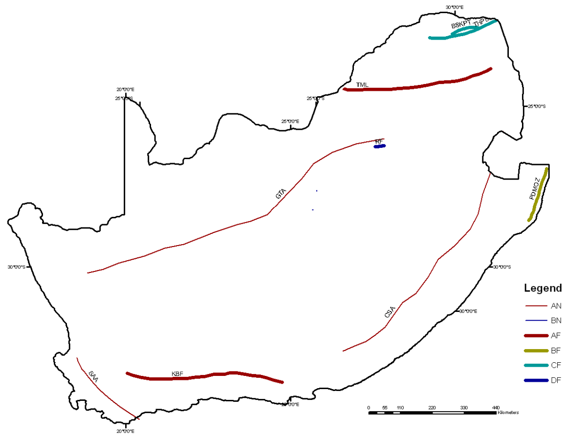
Figure 4 Classification of neotectonic faults and reactivated features. Refer to Table 5 and 6 for symbol meanings and full names of features
