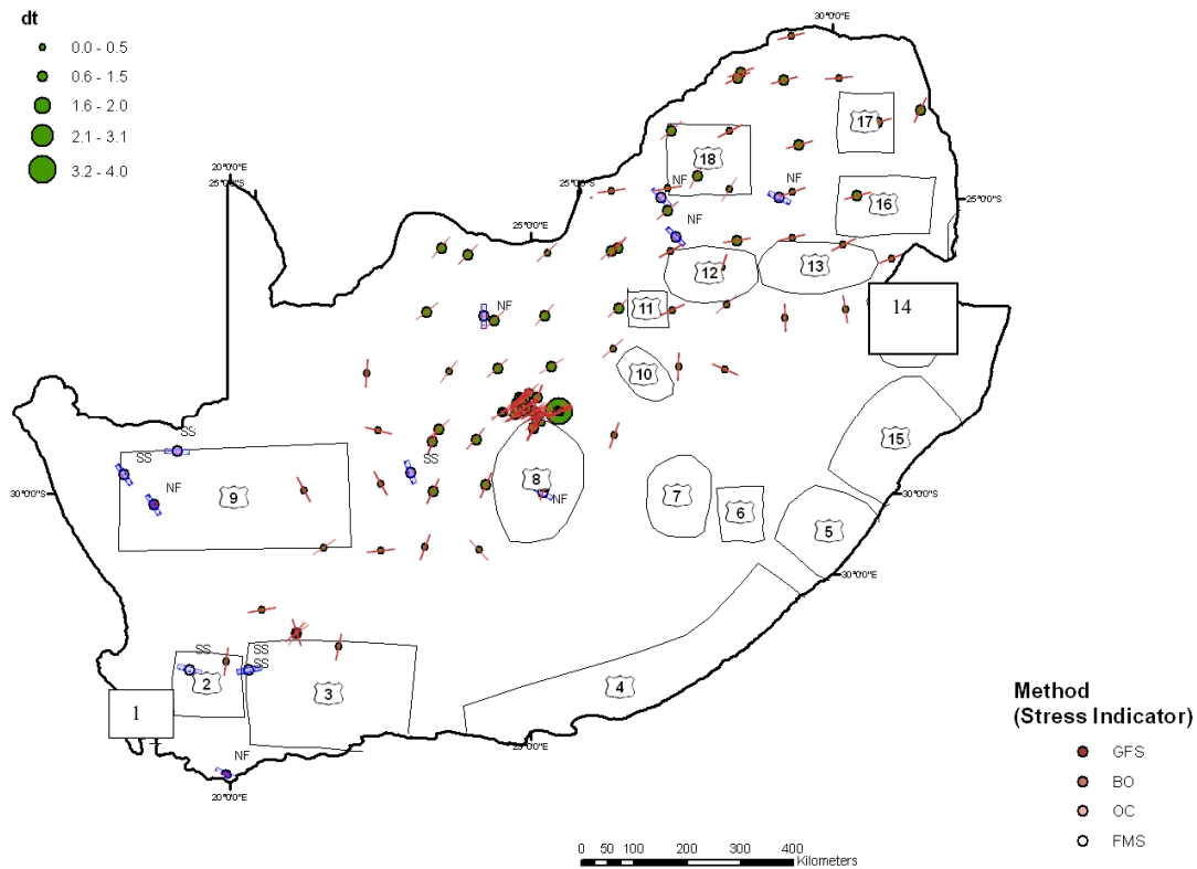
Figure 5 World Stress Map data and data from Bird (2006). Earthquakes forming Clusters 2 and 3 have strike-slip regimes. Earthquakes in Cluster 8 show normal faulting. Other earthquakes towards the north have normal faulting regimes. The method used for calculating stresses are indicated (FMS-Focal mechanism solution, OC-Overcoring, BO-Individual breakouts, GFS- geological fault slip). Orientation of symbol (red line) corresponds to the maximum horizontal stress (SH). SS: strike-slip SH > SV > Sh ; NF: normal faulting SV > SH > Sh .
