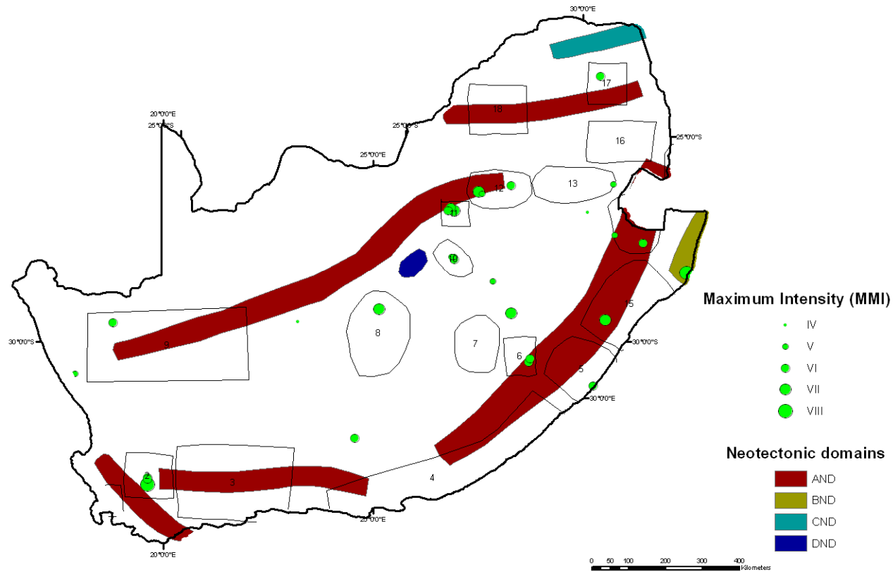
Figure 6 Classified neotectonic domains and CEF schema. The neotectonic domains (AND-DND) are indicated according to the classification scheme implemented.
