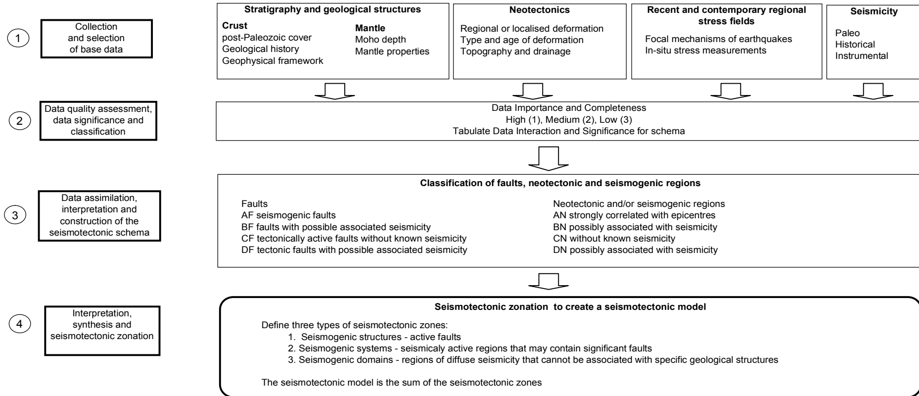
Figure 1 Schematic representation of stages in the creation of a regional seismotectonic model [adapted from Terrier et al. (2000)].
