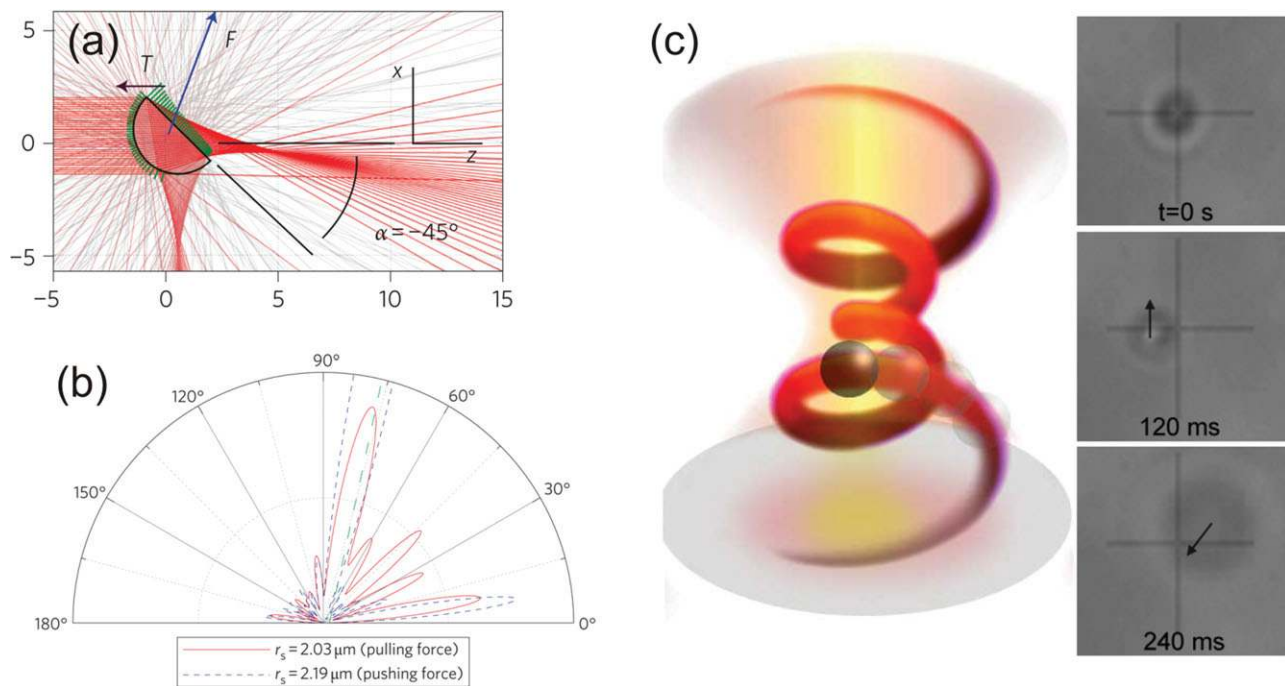
Figure 3 (online color at: www.lpr-journal.org ) Examples of unbalanced optical forces that enable optical manipulation with limited or no trapping: (a) optical lift [76], (b) optical pulling force [67], (c) orbital and translational motion in an ‘optical twister’ [80]. (Images from respective references).
