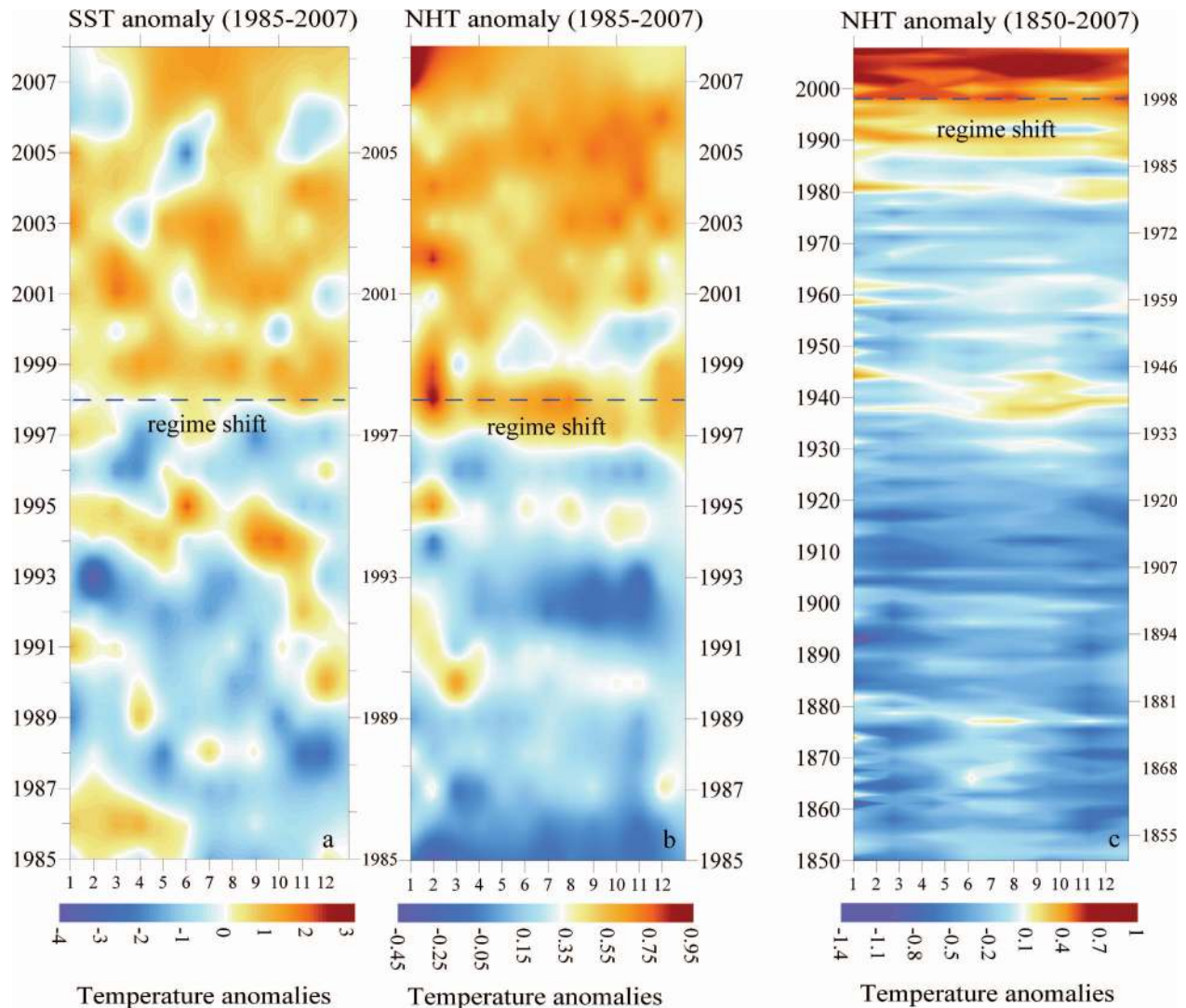
Fig. 2. Long-term or year-to-year changes in both regional and global monthly temperature; on the x -axis the months (1–12) can be seen. (a) Satellite-derived SST (1985–2007) for the Aegean and eastern Ionian Seas. (b) NHT anomalies (1985–2007). (c) NHT anomalies for the period 1850–2007. The blue line in 1998 shows the temperature regime shift, which appeared to be the most abrupt change occurring in the last 158 yr. All the data are expressed as anomalies in order to be comparable; note the different scale in each plot.
