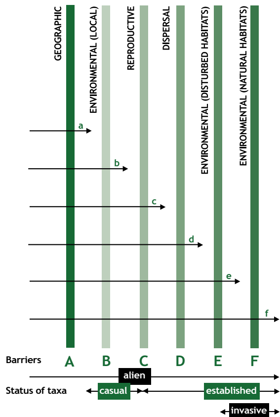
Figure 2. Invasion process (adapted from Richardson et al (2000))
