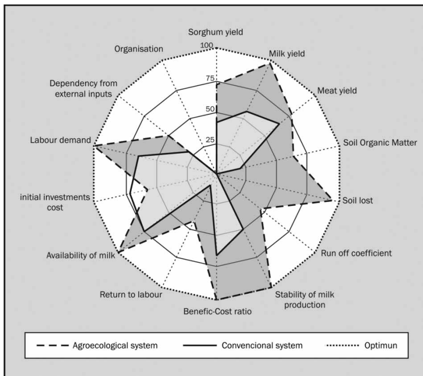
Figure 3 | An AMOEBA diagram with indicators comparing two agrosilvopastoral systems (agroecological versus conventional) in Mexico. Indicators are in original units and as percentages of locally derived optimums Source: Lopez-Ridaura et al. (2002).
