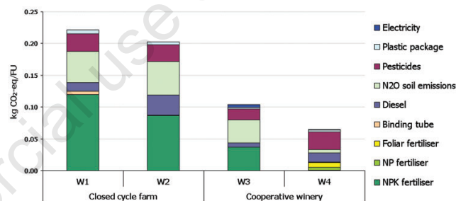
Figure 3. GWP of main processes occurring in the production phase (kg of CO 2 -eq./FU).
