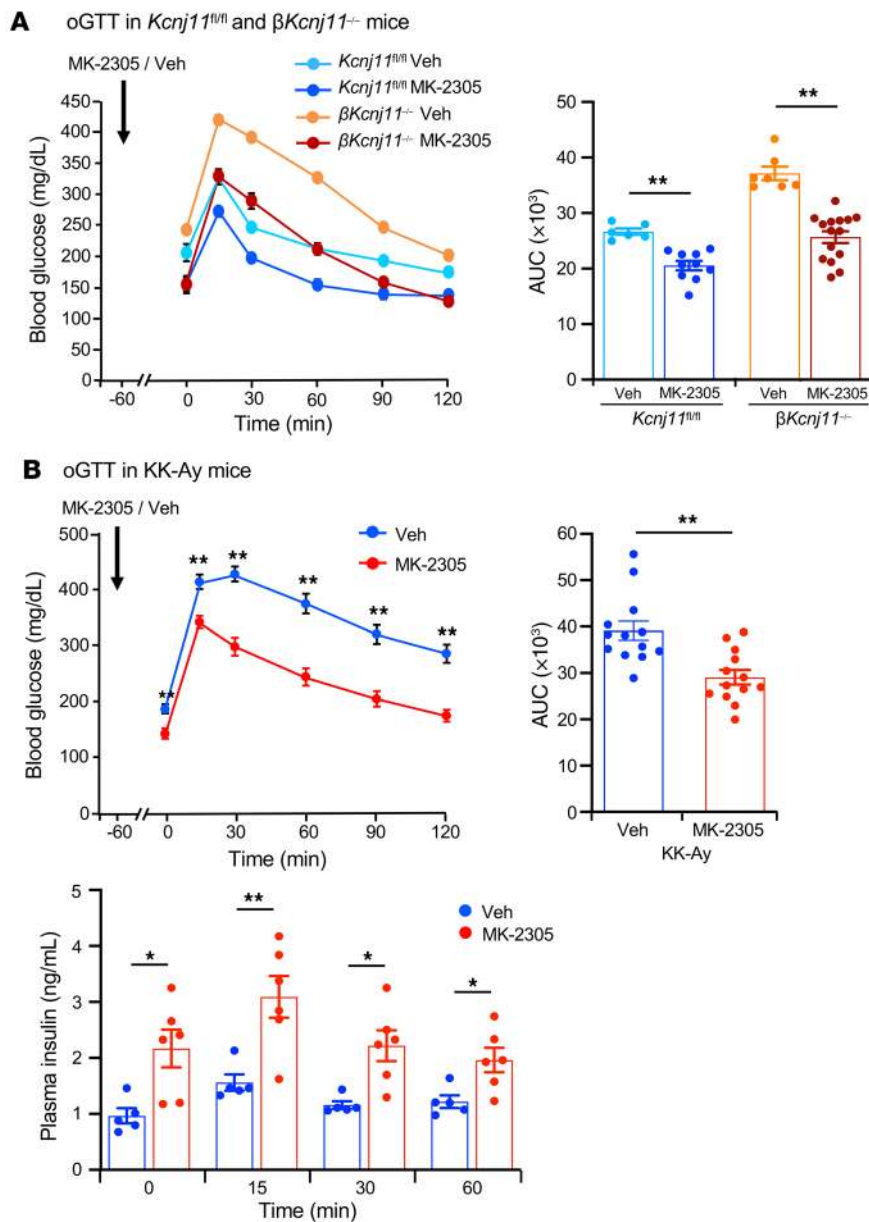
Figure 7. Gq-specific agonist MK-2305 improves glucose tolerance in \beta Kcnj11 -/- mice and KK-Ay mice.
