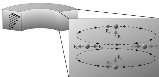
Fig. 1 Schematic illustration of a continuous curved rectangular microchannel in which both the Dean force ( F_D ) and lift force ( F_L ) are present as well as the directions of their applied force on the particles, resulting in a single equilibrium position at the inner wall of the microchannel, where both forces operate in opposite directions.
