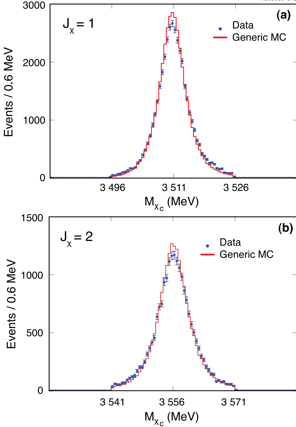
FIG. 4: Plot of the \chi_{cJ} mass as calculated from subtracting the four-vector of the \gamma' from the \psi' four-vector. This variable is not used as a selection criterion because the 1C and 4C kinematic fits ensure that this criterion is redundant with the \chi_{c1} mass selection criterion generated by adding the J/\psi and \gamma four-vectors. (a) J_\chi = 1 and (b) J_\chi = 2 .
