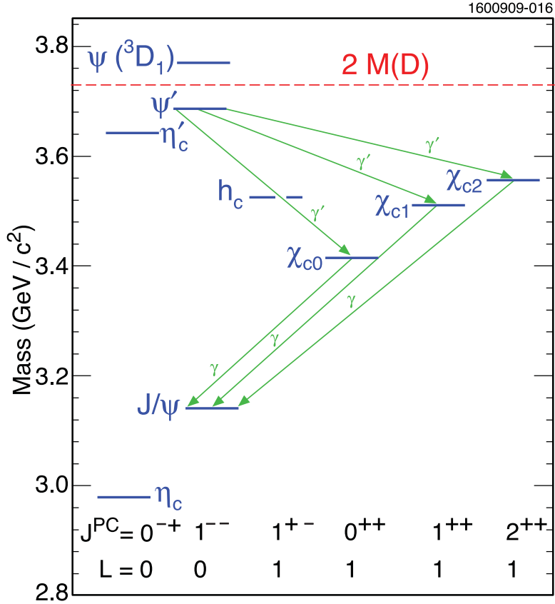
FIG. 1: Charmonium energy levels. Only the transitions studied in this article are shown.
