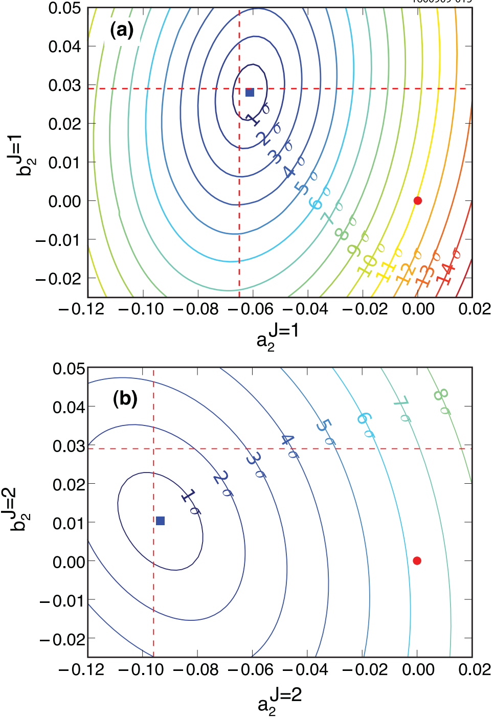
FIG. 5: (a) J_\chi = 1 and (b) J_\chi = 2 log likelihood contours as functions of (a_2, b_2) for two-parameter fits. The fitted values (the solid squares) are (a_2, b_2) = (-0.0611, 0.0281) for J_\chi = 1 and (a_2, b_2, a_3, b_3) = (-0.093, 0.010, 0, 0) for J_\chi = 2 . These are, respectively, 11.1\sigma and 6.2\sigma from pure E1 (the solid circles). The theoretical values to first order in E_\gamma/m_c with \kappa_c = 0 are given by the dashed lines.
