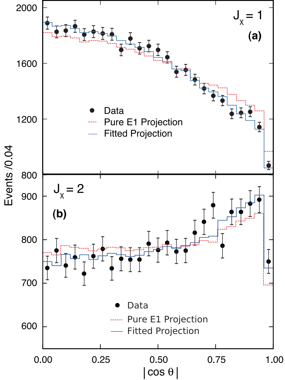
FIG. 6: (a) J_\chi = 1 and (b) J_\chi = 2 projections of \cos \theta after using parity transformations to fold the data set into positive \cos \theta', \phi', \cos \theta_{\gamma\gamma'}, \cos \theta . For J_\chi = 1 ( J_\chi = 2 ) the values of \chi^2/N_{\text{d.o.f.}} for the 25 bin histogram describing the data to correspond with the two-parameter (a_2, b_2) fitted projection are 16.2/22 = 0.74 ( 20.3/22 = 0.92 ) and to correspond with the pure E1 projection are 80.29/24 = 3.35 ( 35.5/24 = 1.48 ). The fitted and pure E1 projections are selected from the same phase space MC sample (via the rejection method), resulting in the correlation of statistical fluctuations in the two projections.
