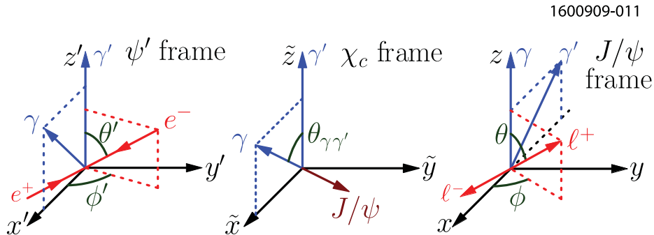
FIG. 2: Reference frames defining the angles used in this analysis. In the \psi' frame, the angles \theta', \phi' are the polar and azimuthal angles of the beam pipe (specifically, the positron's direction) relative to \gamma' defining the z' -axis, and \gamma lying in the x' - z' plane (with a positive x' -component). In the \chi_c frame, the angle \theta_{\gamma\gamma'} is the angle between the two photons. In the J/\psi frame, the angles \theta, \phi are the polar and azimuthal angles of the two leptons (specifically, the positive lepton's direction) relative to \gamma defining the z -axis, and \gamma' lying in the x - z plane (with a negative x -component).
