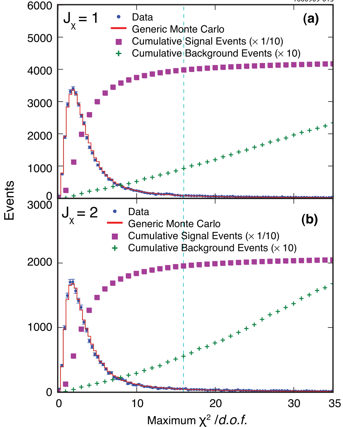
FIG. 3: Maximum reduced \chi^2 in all kinematic fits (including vertex fits) in generic Monte Carlo and data. Events with a maximum reduced \chi^2 below 16 (the dashed vertical line) are kept. Cumulative totals for the number of signal and impurity background events are also plotted for each potential value of a maximum reduced \chi^2 . (a) J_\chi = 1 and (b) J_\chi = 2 .
