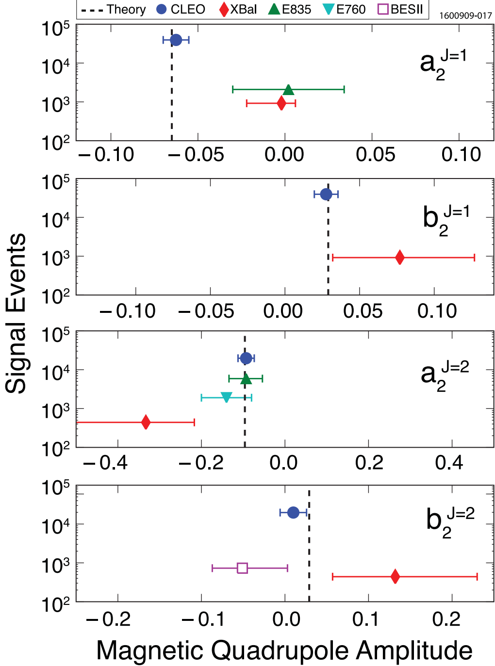
FIG. 7: Experimental values of the magnetic quadrupole amplitudes from this analysis compared with previous experimental values and theoretical expectations. For J_\chi = 2 , results are shown for the two-parameter fit. CLEO-c results from this analysis are solid circles; Crystal Ball results are diamonds [17], the E760 result is a \nabla [18], the E835 results are \Delta 's [12], the BESII result is an open square [19], and the theoretical expectations given by Eqs. (7)–(10) with m_c = 1.5 GeV and \kappa_c = 0 are dashed lines.
