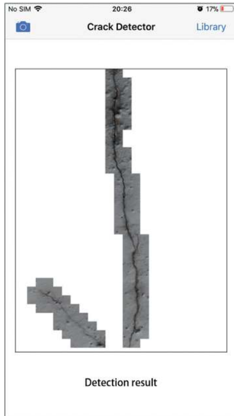
FIGURE 14: Detection result of the Crack Detector.
