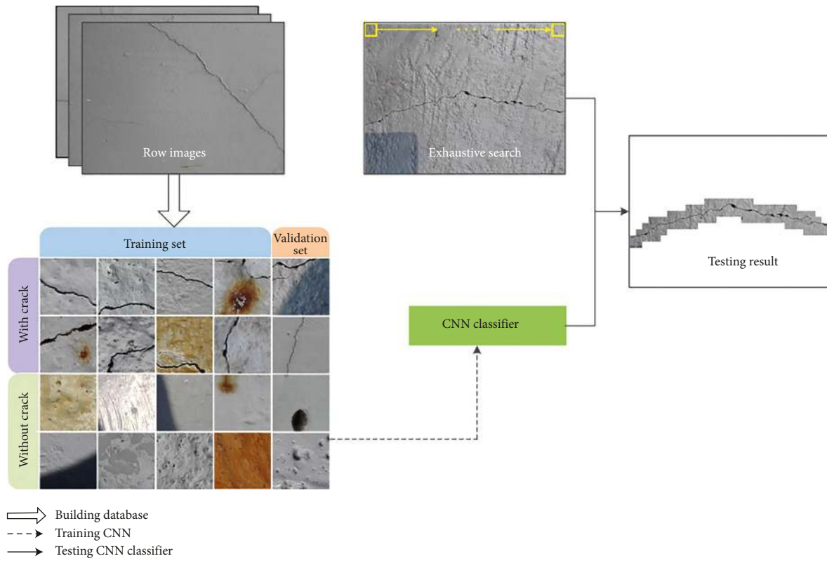
FIGURE 1: Flow chart for detecting cracks using a CNN.
