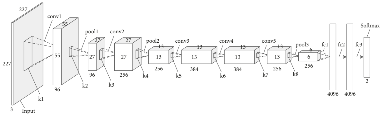
FIGURE 2: Illustration of a CNN's overall architecture. conv# = convolution; pool# = pooling; fc# = full connection; k# = kernel of each operation.
