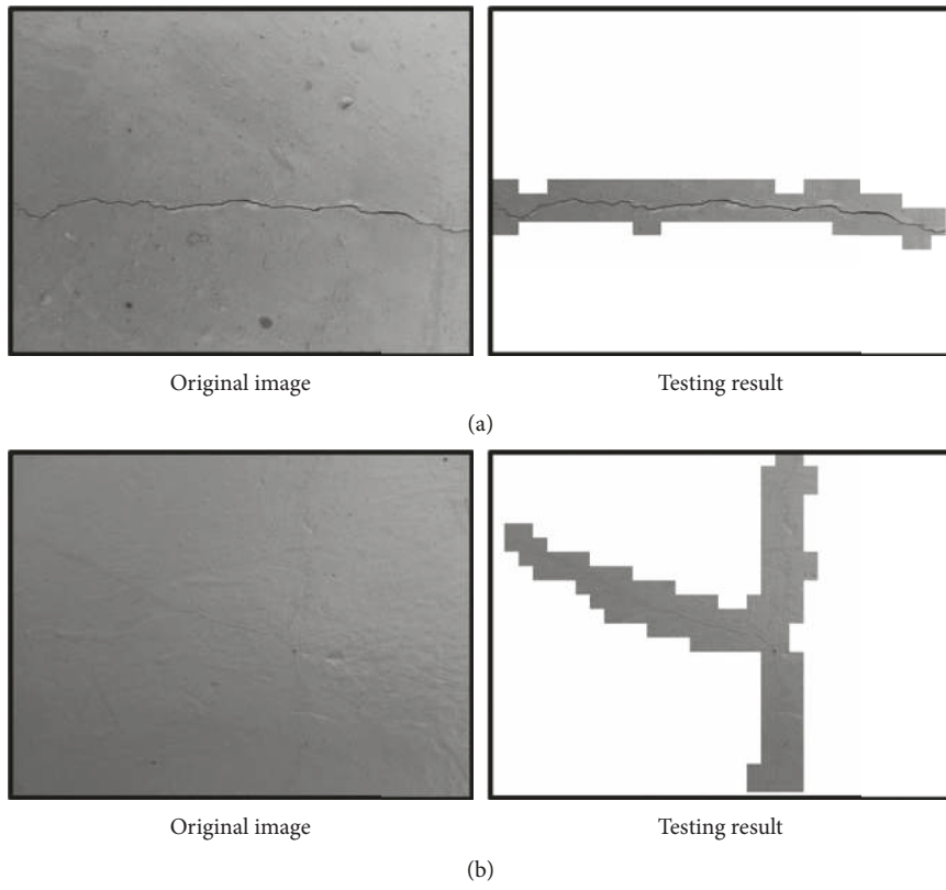
FIGURE 11: Normal surfaces: (a) clear crack; (b) microcracks.
