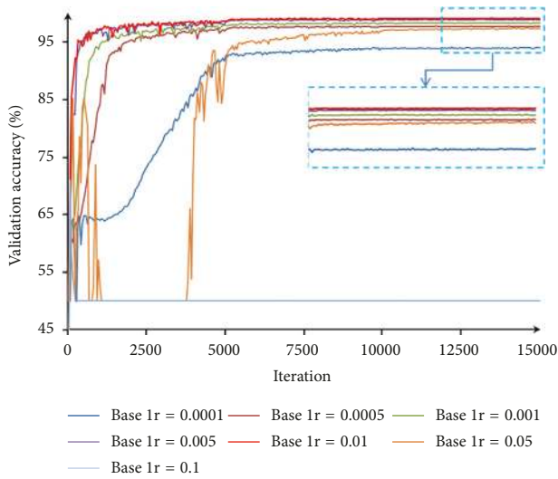
FIGURE 7: Validation accuracies under different base learning rates. base lr = base learning rate.
