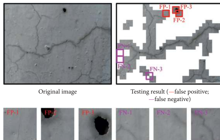
FIGURE 13: Complex and blurry cracks.
