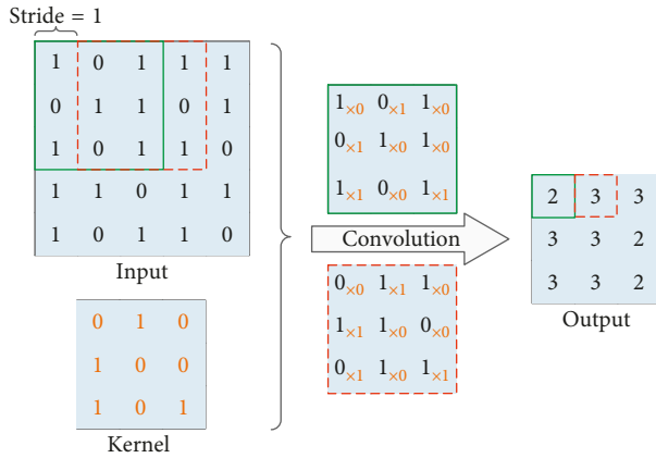
FIGURE 3: Convolution process.
