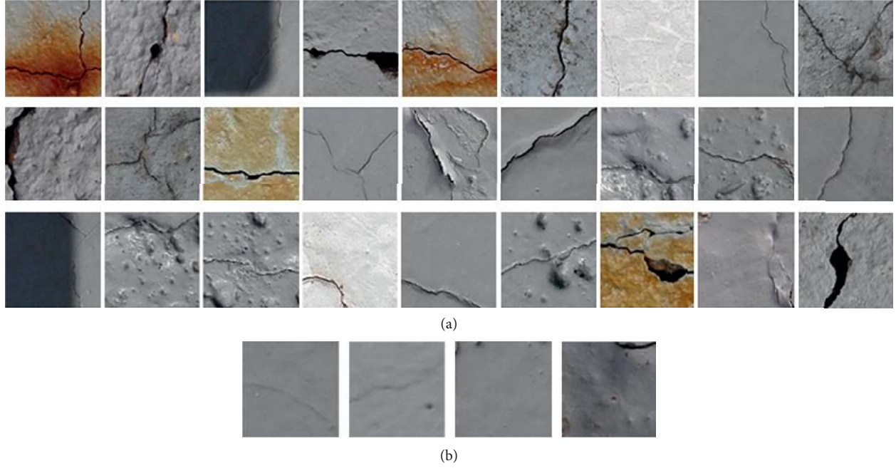
FIGURE 6: Cropped images: (a) images with cracks used for building database; (b) removed images.
