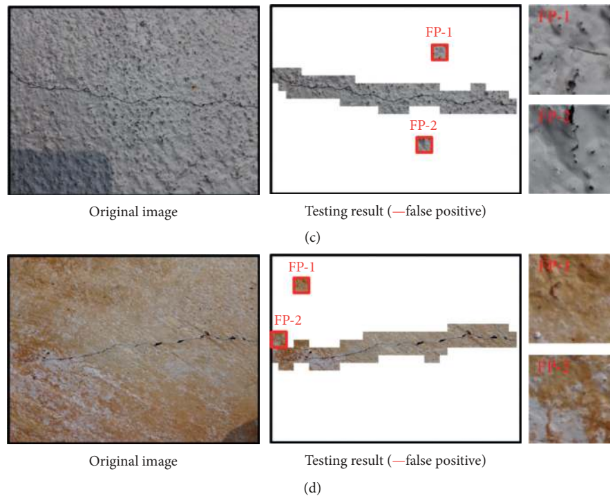
FIGURE 12: Damaged surfaces: (a) shadowed surface; (b) surface with holes; (c) rough surface; (d) rusty surface.
