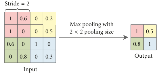
FIGURE 4: Max pooling process.
