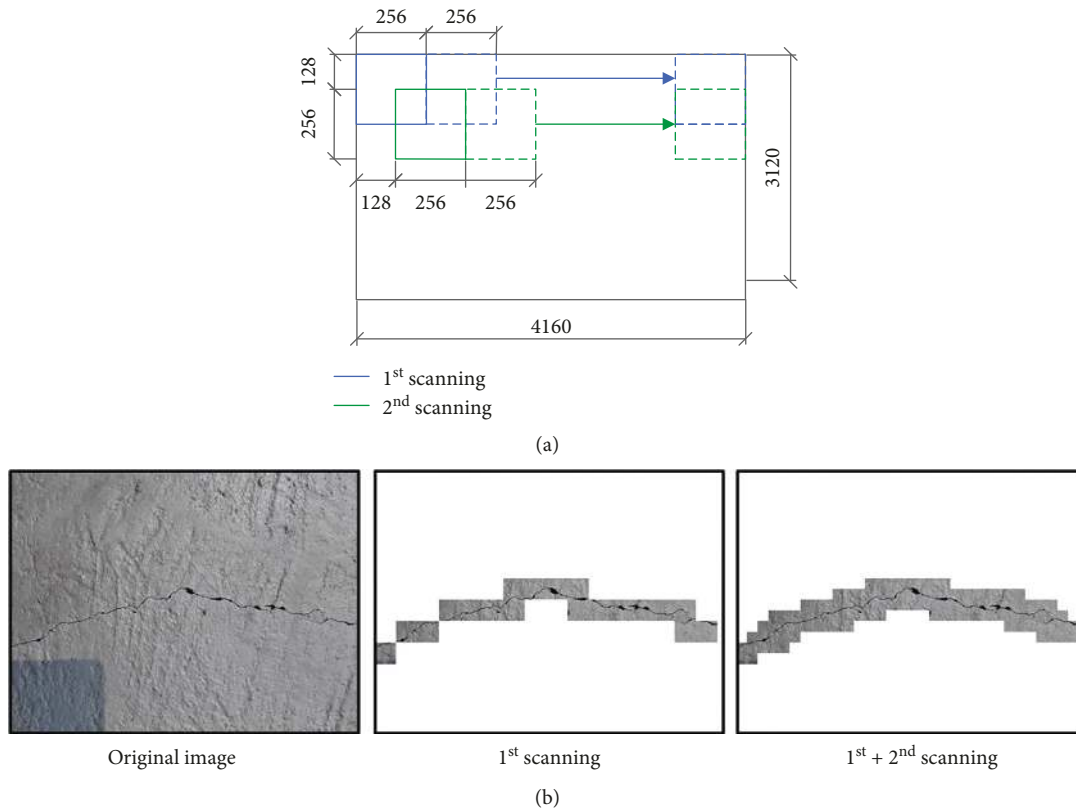
FIGURE 9: Crack detection using exhaustive search: (a) sketch; (b) detection result.
