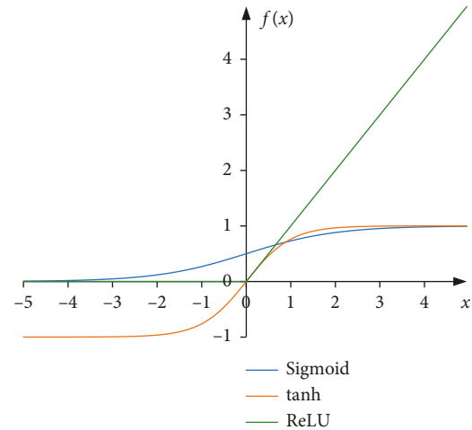
FIGURE 5: Nonlinear activation functions.
