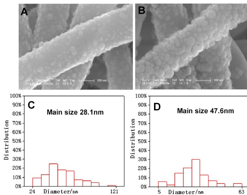
Fig. S1. The representative SEM images (A, B) and size distribution of AgNPs (C, D) of S1 and S2.
