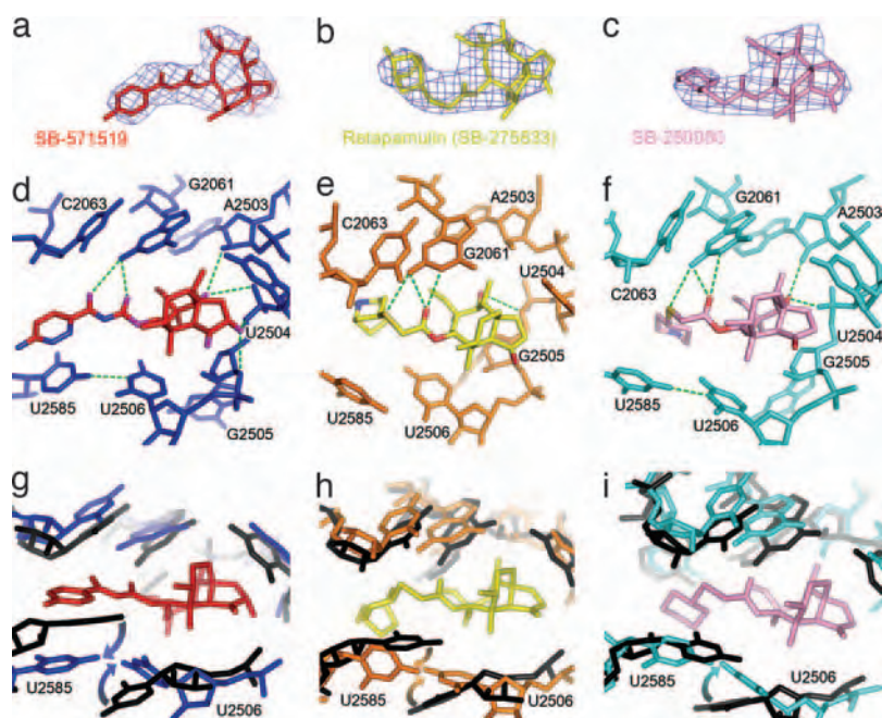
Fig. 2. Selected regions from the crystal structures of the large ribosomal subunit from D. radiodurans complexed with pleuromutilin acyl-carbamate derivative SB-571519 (in red: a , d , and g ) and two sulfanyl-acetate derivatives retapamulin (SB-275833) (in yellow: b , e , and h ) and SB-280080 (in pink: c , f , and i ) at 3.50, 3.66, and 3.56-Å resolution, respectively. ( a–c ) 2F_o - F_c electron density maps, contoured at 1.5\sigma level. ( d–f ) Interactions between pleuromutilin derivatives and 23S rRNA (the 23S rRNA bound conformation is shown in dark blue for SB-571519, orange for SB-275833, and cyan for SB-280080). All show H-bonds between G2061 and pleuromutilins' C14 extension and the possibility of H-bond between C11 hydroxyl and G2505 phosphate. In SB-571519 and SB-280080 complexes, C11 hydroxyl may serve as acceptor in an additional H-bond with the OH group of A2503 O2', and a nontypical H-bond is observed between U2585 and U2506. ( g–i ) Induced-fit mechanism promotes pleuromutilins binding (color code as in d–f ). In all, the unbound 23S rRNA (PDB ID code 1NKW) is black, and the pleuromutilin-bound conformations are colored. On binding, U2585 translates away from the C14 extension and U2506 rotates toward the pleuromutilin and thus closes tightly the binding pocket. H-bonds ( d and f ) or other interactions ( e ) between the two shifted nucleotides may further stabilize the rRNA conformation at the bound state.
