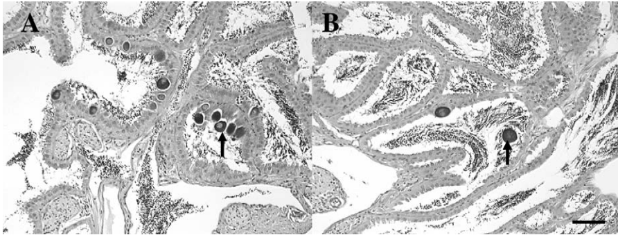
FIGURE 6.—Testicular oocytes in smallmouth bass. Two sections (A) and (B) illustrating oocytes (arrows) could be observed free in the lumen of the seminiferous tubules during and after spawning. Bar = 50 \mu m. H&E stain used.
