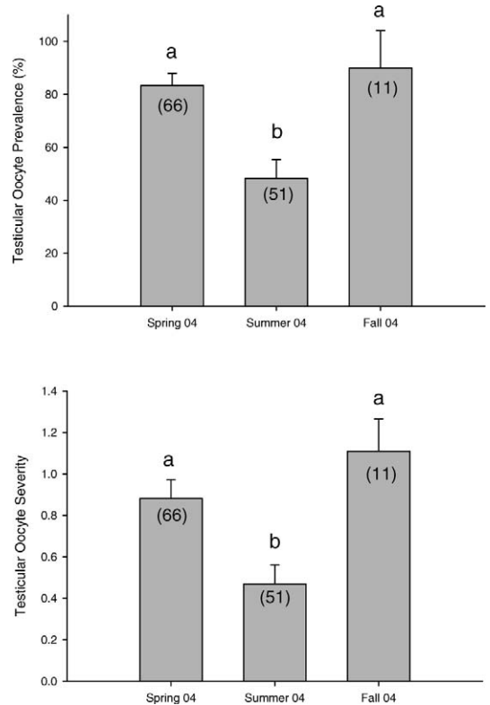
FIGURE 5.—Seasonal prevalence and severity of testicular oocytes in male smallmouth bass from the South Branch of the Potomac River. Bars labeled with the same letter are not significantly different. Numbers in parentheses indicate the number of males collected each season.
