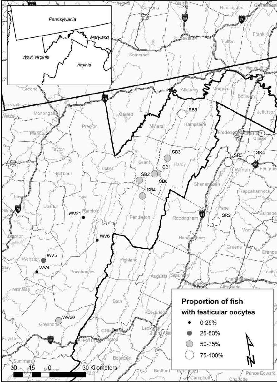
FIGURE 1.—Site locations and prevalence of testicular oocytes in smallmouth bass in the Potomac River drainage and adjacent rivers.
