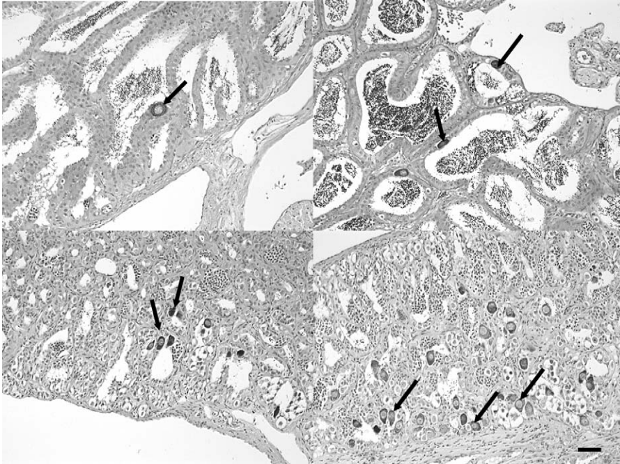
FIGURE 3.—Testicular oocyte severity index for evaluation of smallmouth bass gonads. ( upper left ) Severity rank 1, single oocyte. Individual oocyte (arrow) noted in field of view. ( upper right ) Severity rank 2, multifocal. More than one oocyte per field of view, but oocytes (arrows) are not closely associated. ( lower left ) Severity rank 3, cluster. Groups (2–5) of oocytes (arrows) closely associated with each other. ( lower right ) Severity rank 4, zonal. Multiple clusters or more than five closely associated oocytes. Bar = 50 \mu m. H&E stain used.
