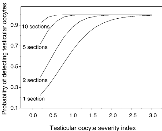
FIGURE 4.—Probability of detecting testicular oocytes in smallmouth bass as a function of the number of sections examined and severity.
