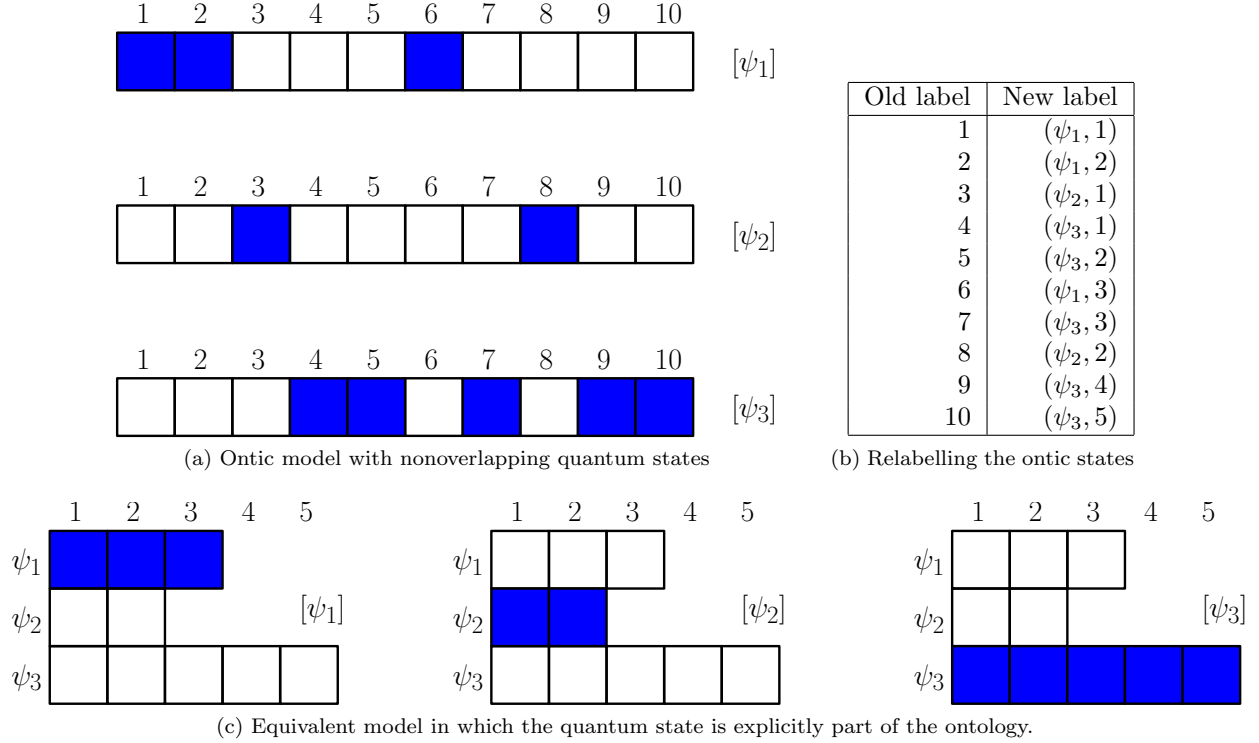
Figure 9: In an ontological model, if the probability measures corresponding to distinct quantum states do not overlap, then the ontic states can be relabelled such that the quantum state is explicitly part of the ontology. Fig. (a) depicts the measures corresponding to three quantum states on a discrete ontic state space consisting of the integers from 1 to 10. Blue boxes indicate the ontic states on which the measures have support. Fig. (b) shows a one-to-one map to a new ontic state space in which the quantum states are an explicit part of the ontology. The result is shown in Fig. (c).
