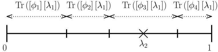
Figure 7: Example of the response functions of the Bell model for a measurement in \mathbb{C}^4 . The unit interval is divided into 4 subintervals of length \text{Tr}([\phi_j][\lambda_1]) . If \lambda_2 is in the j th interval then the outcome will be [\phi_j] . In the case depicted, the outcome is [\phi_3] .
