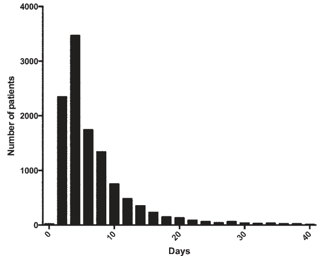
FIG. 1. Histogram showing the distribution of length of stay in the study population. The 99th percentile of hospital stay was 38 days; however, 104 patients had hospital stays greater than 40 days, with the longest being 369 days.
