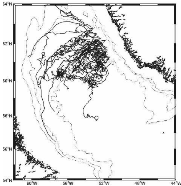
FIG. 11. Irminger Ring tracks for years 6 and 7 in the REBAT experiment. Dashed lines indicate the 1000-, 2000-, and 3000-m isobaths.
