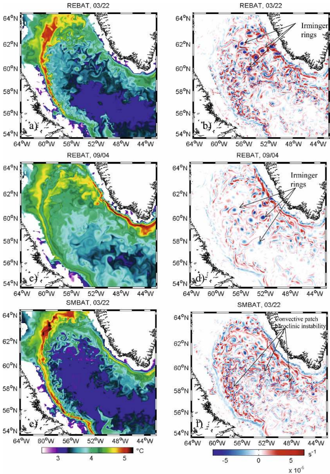
FIG. 10. Snapshots of (left) potential temperature and (right) relative vorticity at -182 \text{ m} in the western part of the domain in March and September of year 8. (a)–(d) REBAT; (e), (f) SMBAT.
