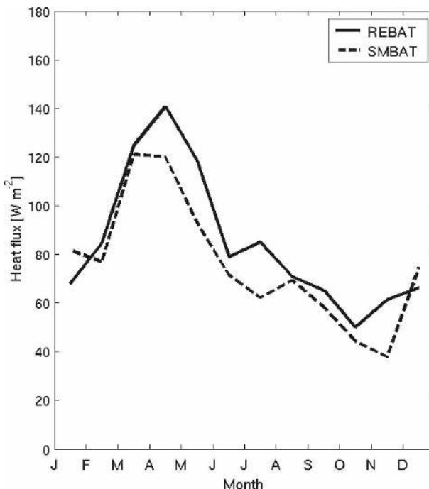
FIG. 18. Monthly lateral heat flux in the interior ( \text{W m}^{-2} ) averaged for years 6 to 10.
