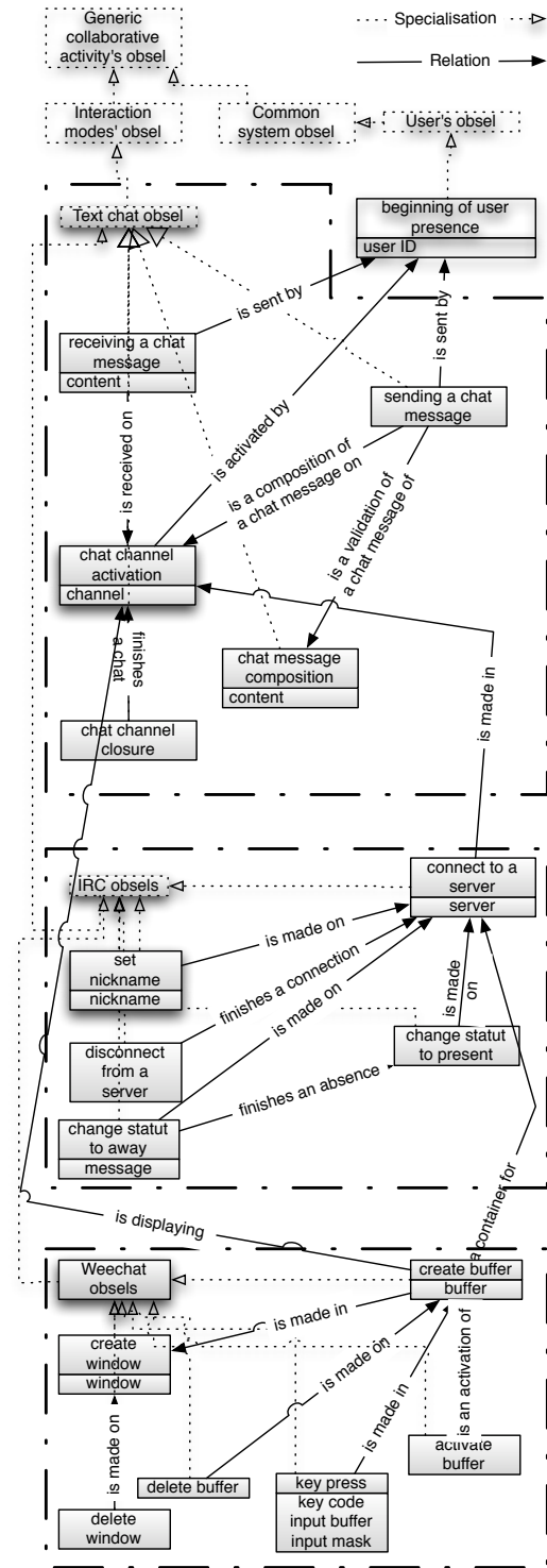
Fig. 8. Exerpt from the WeeChat’s specific trace model
