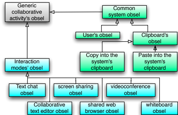
Fig. 4. Structure of the generic trace models for synchronous collaborative activities; specific obsels are not all detailed here
