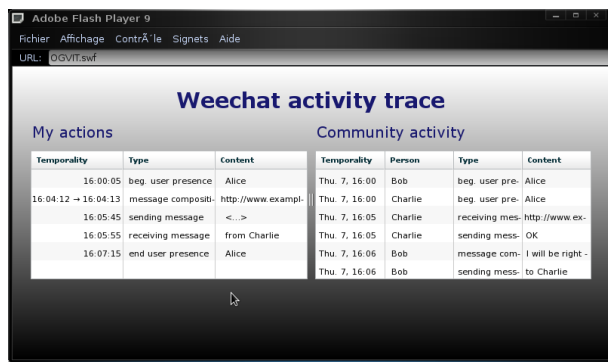
Fig. 9. Screenshot of the Tool for generic interactive visualisation of traces. It is displaying a rendering of Alice's trace, as well as the traces collected from Bob and Charlie.
