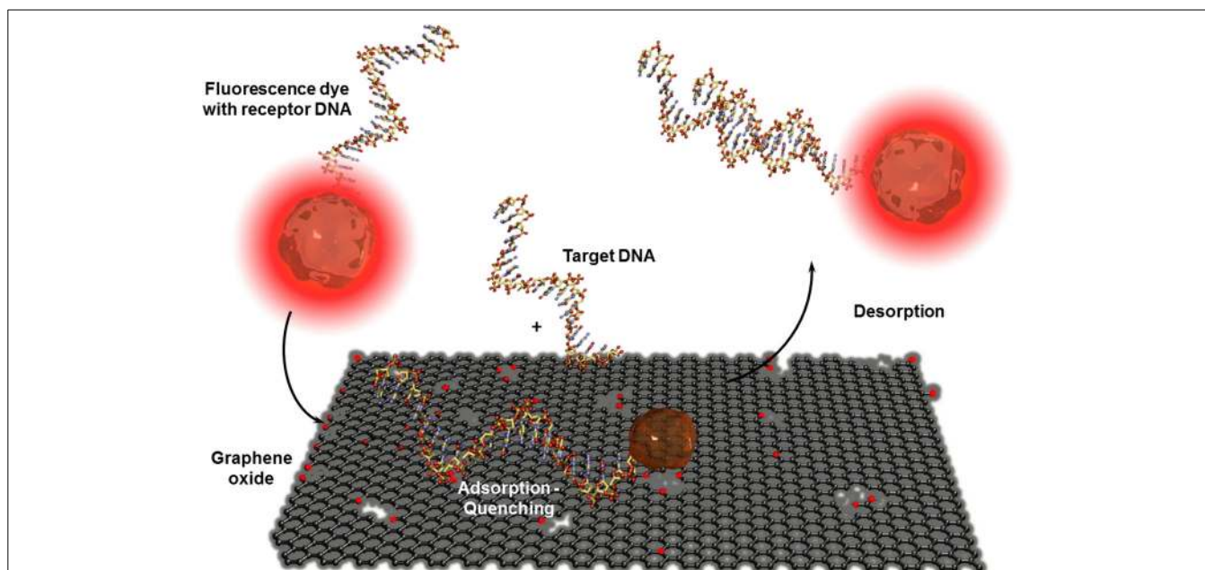
FIGURE 9 | Adsorption and desorption of a fluorescence dye modified receptor DNA on graphene oxide before and after hybridization with the corresponding target DNA. Graphene oxide quenches the fluorescence of
