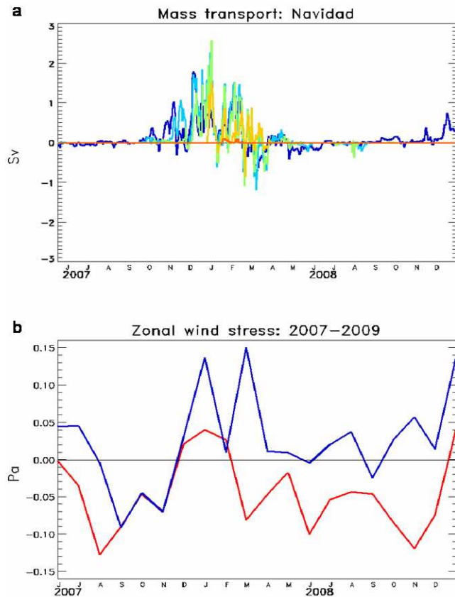
Fig. 18. (a) Transport (Sv) of the poleward flow for water mass warmer than 13.0^{\circ}\text{C} and saltier than 35.7\text{ psu} at 43.24^{\circ}\text{N} (blue), 7.61^{\circ}\text{W} (turquoise blue), 6.2^{\circ}\text{W} (green), 3.8^{\circ}\text{W} (yellow) and 44.4^{\circ}\text{N} (orange). (b) Meridional wind stress \tau_y (Pa) off western Iberia (red) and of the zonal wind stress \tau_x off northern Iberia (blue). Boxes chosen for the spatial average of \tau_x and \tau_y have been chosen following the study of Le Cann and Serpette (2009).
