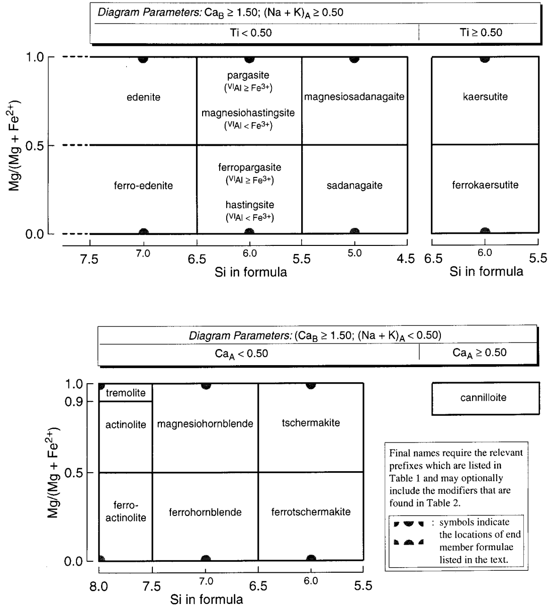
FIG. 3. Classification of the calcic amphiboles.
