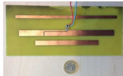
Fig. 6. Rectenna, consisting of a 50 \Omega receive antenna, a lumped element matching network, and a voltage-doubling rectifier. DL = 106 mm, DW = 8 mm, DD = 8 mm, RL = 167 mm, RW = 5 mm, RD = 20 mm, FL = 158 mm, FW = 10 mm, t = 39 mm, b = 2 mm, and g = 1 mm. The copper thickness is 70 \mu\text{m} . The FR4 board ( \epsilon_r = 4.28 , \tan\delta = 0.0016 ) is 1.6 mm thick.
