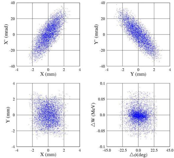
Figure 11: Particle distribution behind the RFQ using the input distribution shown in Figure 8 ( \epsilon_{x,rms}=0.62 \pi \text{ mmmrad} ; \epsilon_{y,rms}=0.62 \pi \text{ mmmrad} , \epsilon_{z,rms}=0.21 \pi \text{ deg MeV} ).
