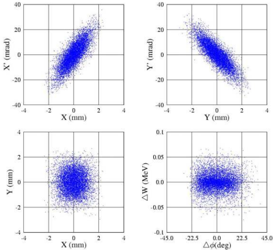
Figure 10: Particle distribution behind the RFQ for the input distribution shown in Figure 7 ( \epsilon_{x,rms}=0.35 \pi \text{ mmmrad} ; \epsilon_{y,rms}=0.35 \pi \text{ mmmrad} , \epsilon_{z,rms}=0.19 \pi \text{ deg MeV} ).
