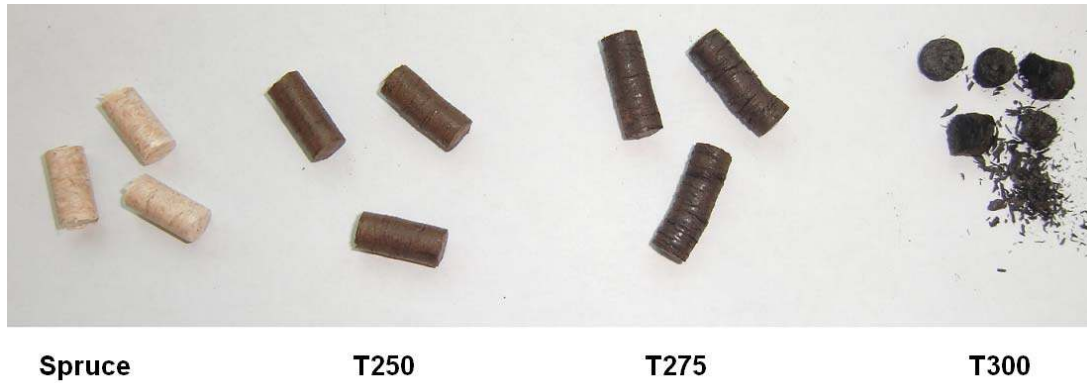
Figure 5. Pellets made from spruce and torrefied spruce. From left to right: Spruce and torrefied spruce at 250, 275 an 300 °C.
