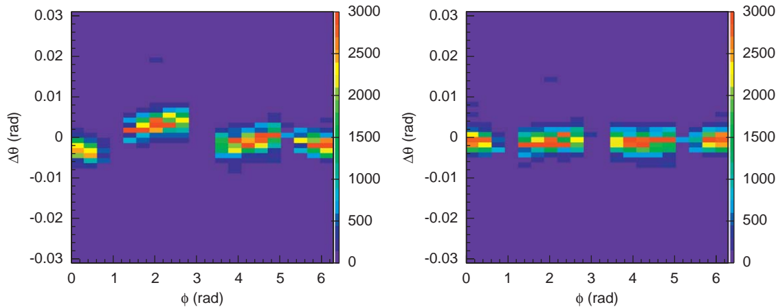
Fig. 6. Difference of the measured Cherenkov angle and expected angle ( \Delta\theta_C ) as a function of the angle around the Cherenkov ring \phi_C with a C_4F_{10} radiator after preliminary mirror alignment (left) and full alignment (right).
