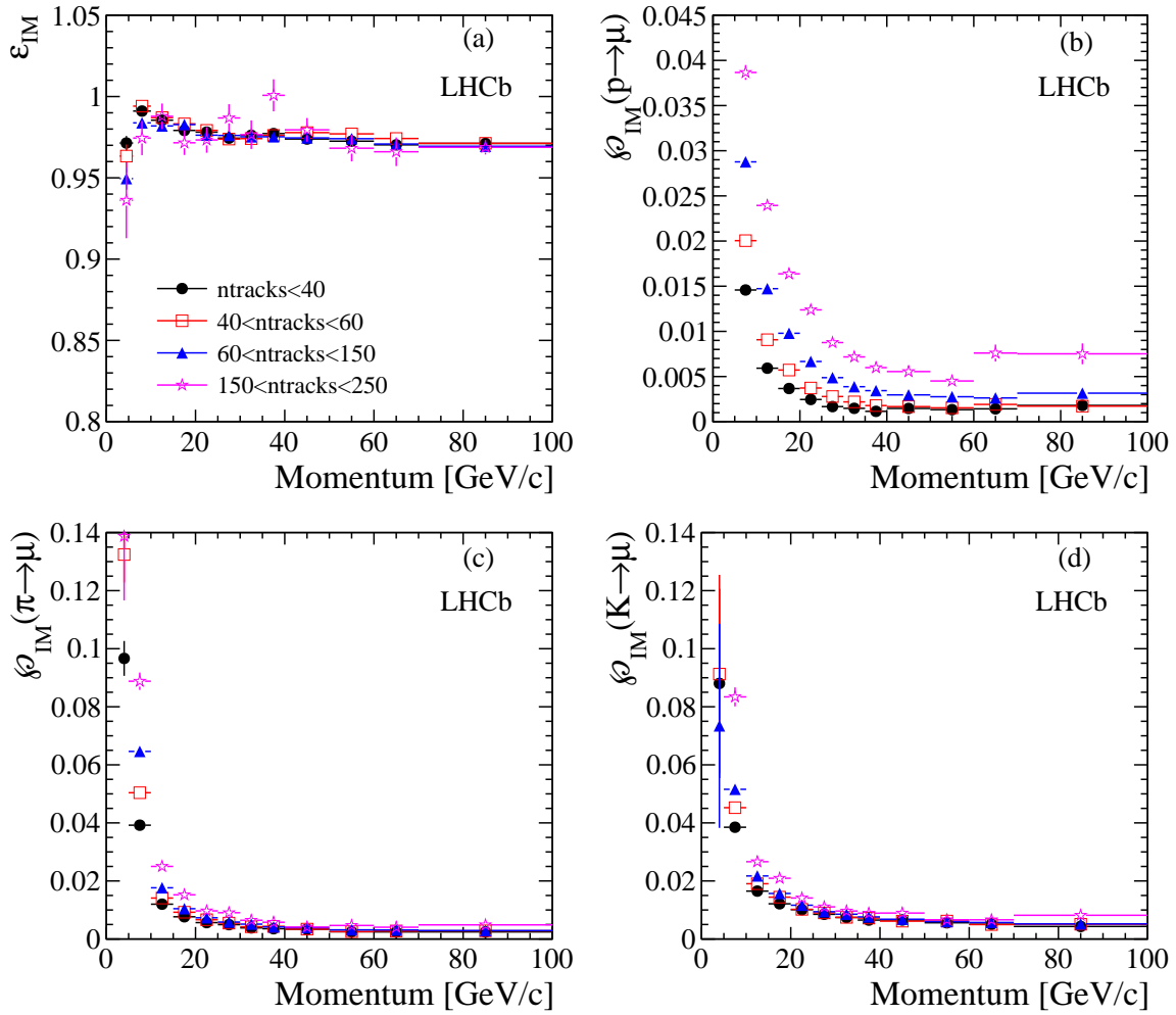
Figure 6. IsMuon efficiency \varepsilon_{IM} (a) and \phi_{IM} for protons (b), pions (c) and kaons (d) as a function of momentum for different ranges of the number of trajectories reconstructed in the event ( n_{tracks} ).
