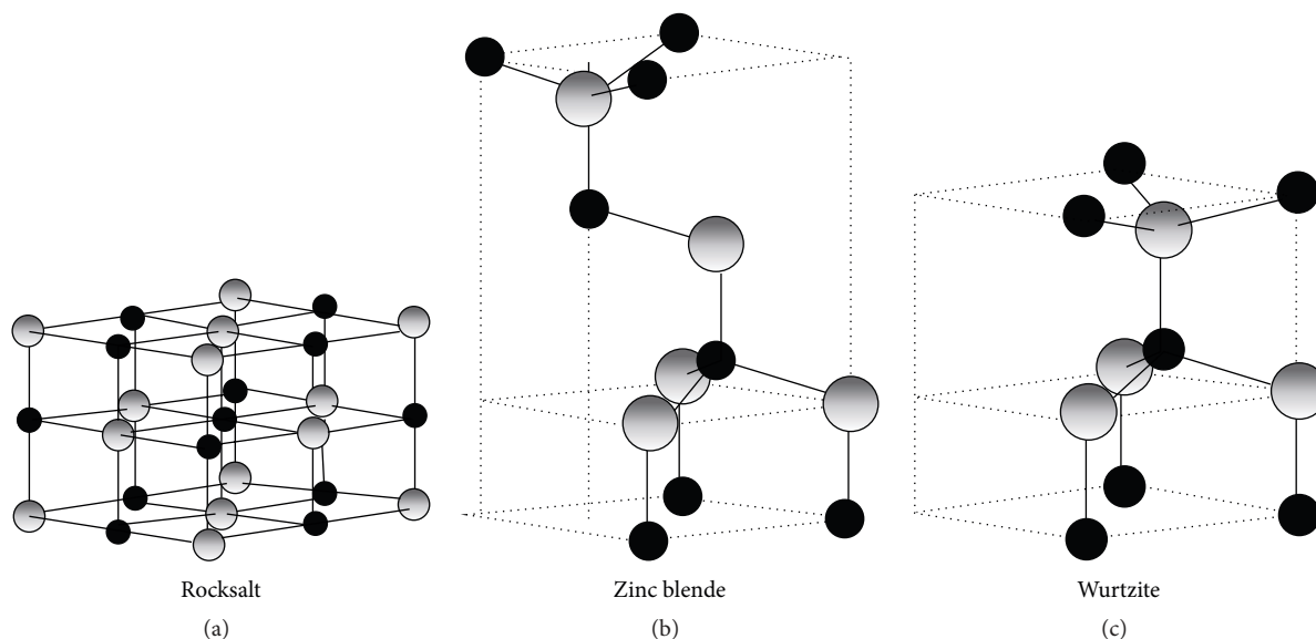
FIGURE 1: Stick and ball representation of different ZnO crystal structures: (a) cubic rocksalt, (b) cubic zinc blende, and (c) hexagonal wurtzite. The shaded gray and black spheres denote Zn and O atoms, respectively [96].
