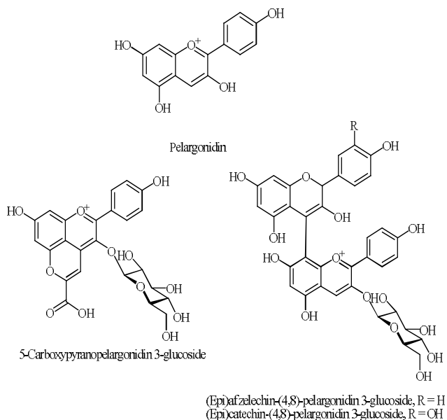
Fig. 8: Chemical structures of anthocyanin found in strawberry.
