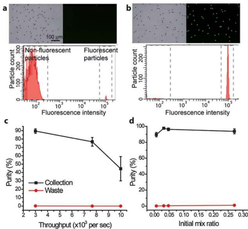
Fig. 5. PLACS sorting results. (a) Mixed 10 μm green fluorescent and non-fluorescent polystyrene microspheres before sorting. Initial mix ratio = 0.0087. (b) Collected sample after sorting with a final mix ratio = 9.61. Fluorescent microsphere concentration was enriched by a factor of 1105. (c) Sort purity at different sorting speeds ranging from 3000 to 10 000 microspheres s -1 . High purities (90 ± 3% (mean ± s.d.)) of the sorted particles were obtained at a sorting throughput of 3000 particles s -1 . The collection purity measured at the highest speed tested (10 000 particles s -1 ) was 45 ± 15%. The sort purity decreased at higher throughputs as the average distance between adjacent particles shortened. In these experiments, green fluorescent particle concentrations were kept constant (5.7 × 10 4 ml -1 ) while non-fluorescent particle concentrations were increased accordingly to obtain the target throughput. (d) Sort purity at different initial mix ratios ranging from 0.001 to 0.27 (unsorted purity 1% to 21%). At the initial mix ratio of 0.27, measured collection target particle purity was 94 ± 3% and waste target particle purity was 1 ± 0%. Sorting speed was kept at 3000 particles s -1 .
