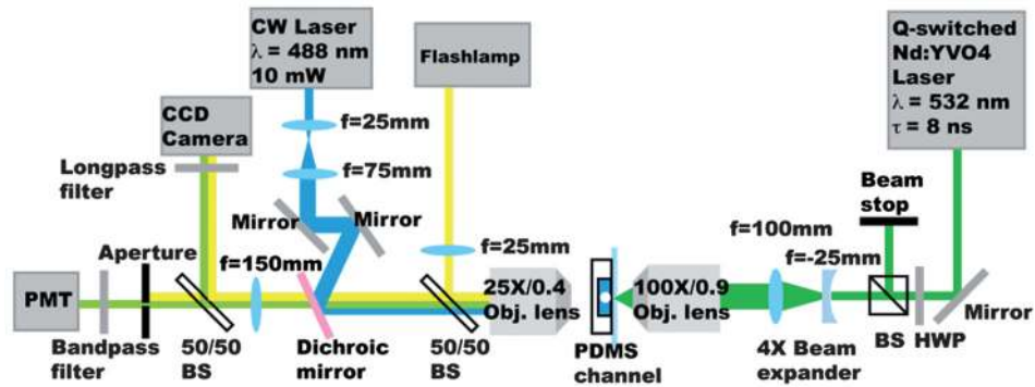
Fig. 4. PLACS experimental setup. For cavitation bubble induction, we used a Q-switched, 8ns pulsewidth Nd:YVO4 laser. The pulsed laser beam was focused by an objective lens (100 \times , NA 0.9) into the pulsed channel. Sample fluorescence was detected by a photomultiplier tube and sampled using a DAQ card and integrated every 10 \mu s. FPGA logic was programmed using LabView to perform real-time detection, threshold comparison and timed triggering of the pulsed laser.
