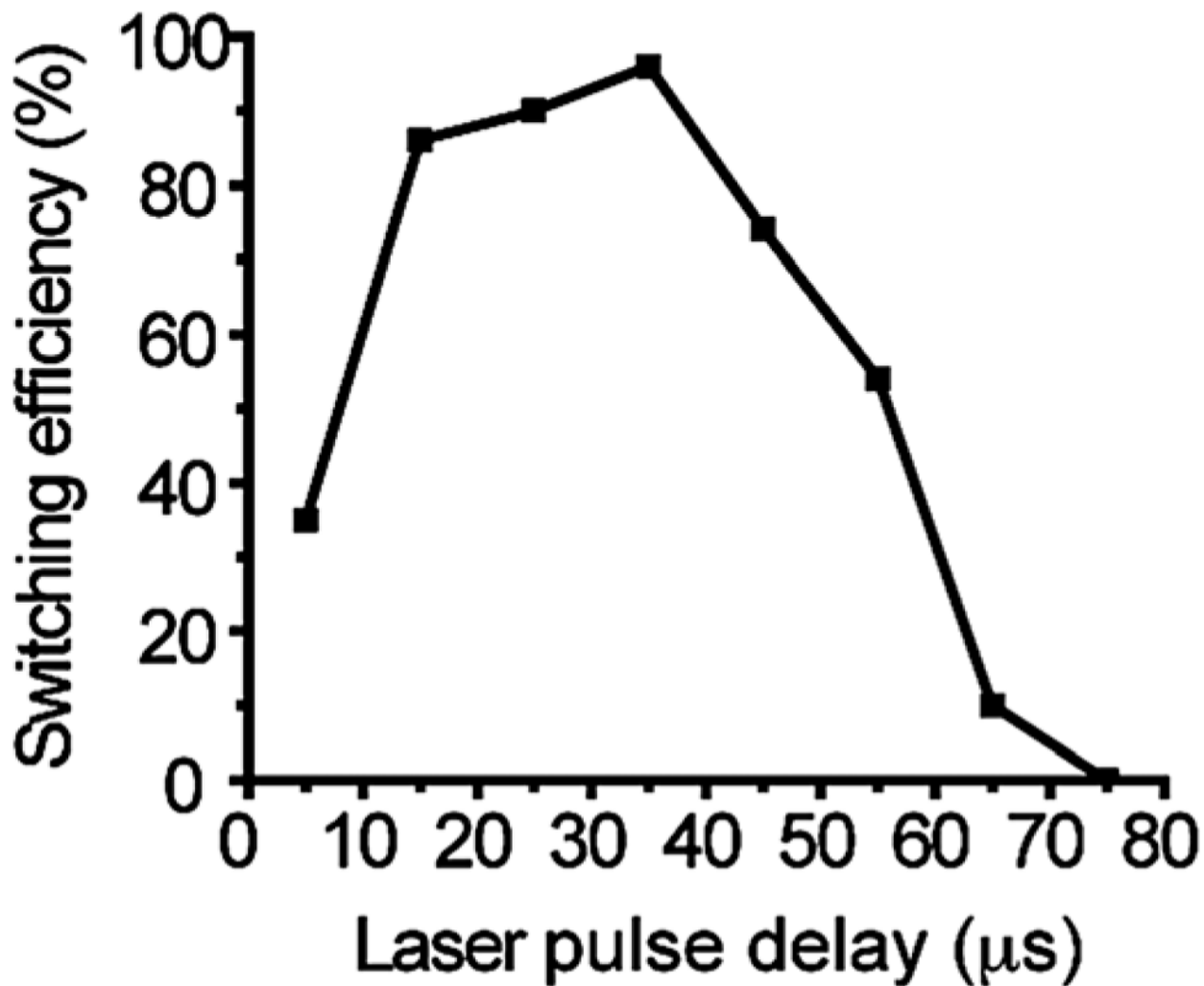
Fig. 3. Switching window and optimum object switching delay. Particle switching efficiency was measured at different laser pulse delays ranging from 5 to 75 \mu\text{s} after detection. The highest switching efficiency of 96% was obtained at a delay of 35 \mu\text{s} and decreased to 0% at 75 \mu\text{s} . The perturbation range of neighboring objects is \sim 60 \mu\text{m} , estimated by the particle speed ( 0.8 \text{ m s}^{-1} ) and the 75 \mu\text{s} window. The distance between the detection region and Y junction was 50 \mu\text{m} . The sorting efficiency was obtained by analyzing particle traces from 50 switching events for each delay condition.
