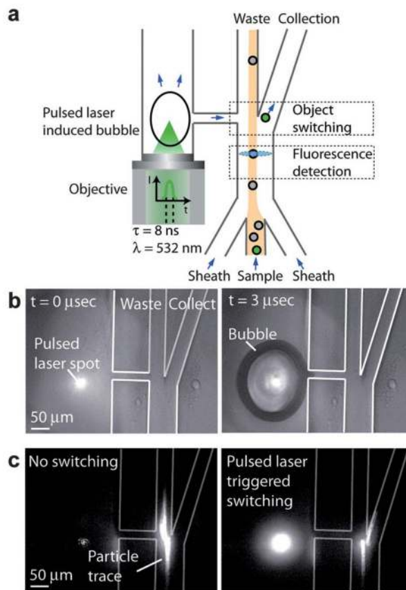
Fig. 1. PLACS operation. (a) Schematic of the cell sorter. The sample flow is hydrodynamically focused into the waste channel. As the desired object flows through the fluorescence detection region upstream from the Y junction, the laser pulse is triggered after an optimum delay and induces a cavitation bubble in the adjacent pulsed channel. The bubble expansion produces a high-speed liquid jet that deflects the desired sample towards the collection channel for sorting. (b) Time-resolved images of the cavitation bubble generated by the focused pulsed laser beam in the micro-fluidic cell sorter. (c) Fluorescent particle switching in PLACS. Without switching, the particle flows towards the left waste outlet. With fluorescence activated switching, a laser pulse was triggered and the particle was sorted into the collection outlet on the right.
