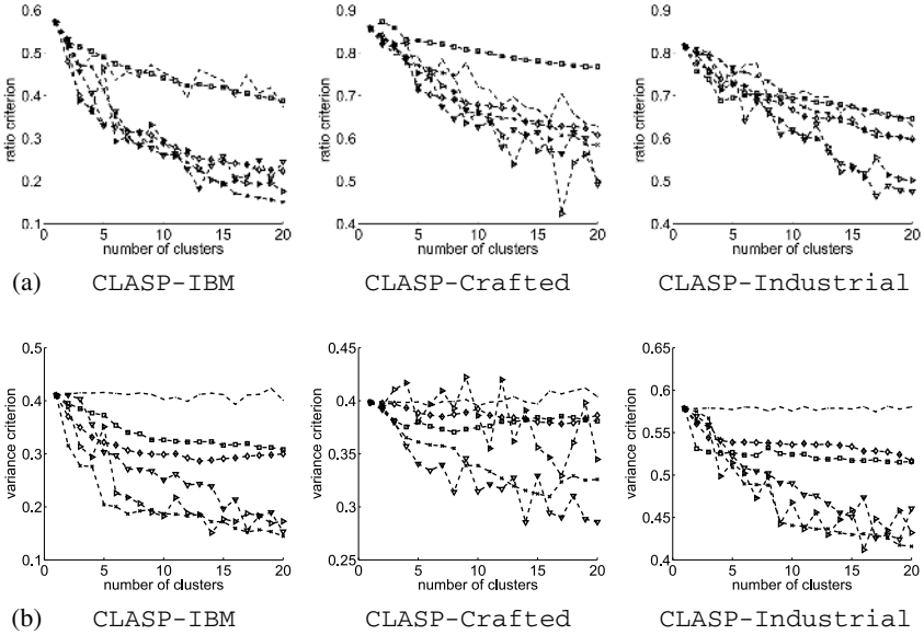
Fig. 2. Q_{Ratio} (a) and Q_{Var} (b) for a varying number of clusters; – random, × Agglomerative Clustering, ▷ Gaussian Mixture, □ Agglomerative Clustering with Q_{Var} optimization, ◇ Agglomerative Clustering with Q_{Ratio} optimization, ▽ feature-based K-Means clustering
