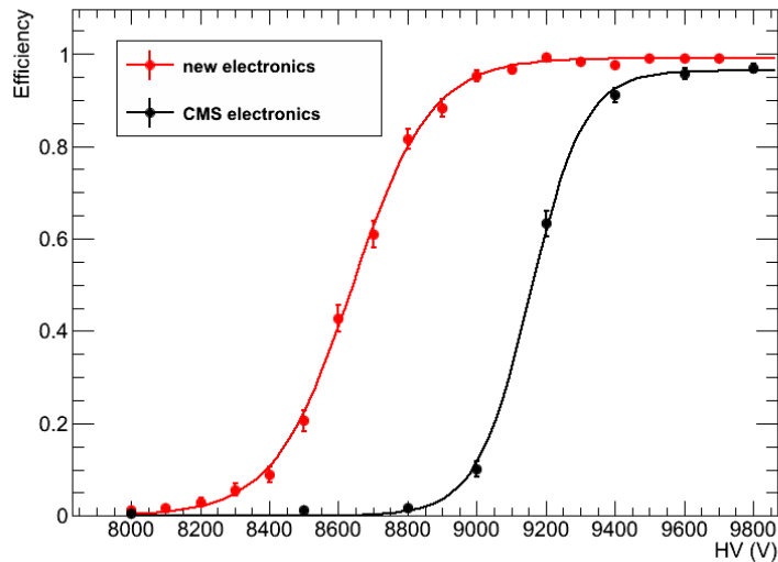
Figure 5. Left: block diagram of INFN amplifier where R1 is the input impedance resistance. C1 \ll C2 and R1 \ll R2 are the conditions for the circuit to work properly. Right: efficiency plateaus for the cases of the standard CMS RPC front-end electronics and new INFN prototype electronics. A lower charge crossing the RPC gap is indicated by the shift of the plateau toward lower voltages leading to an improved rate capability of the RPC.
