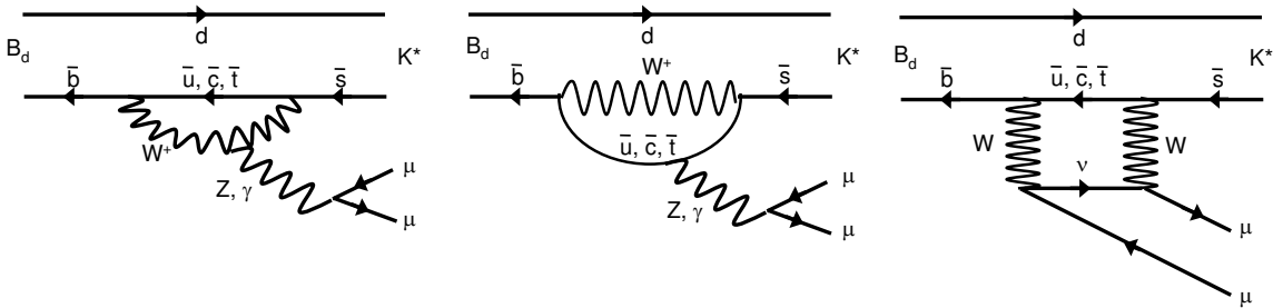
Figure 1: Dominant Standard Model Feynman diagrams for the B_d \rightarrow K^{*0} \mu^+ \mu^- decay.
