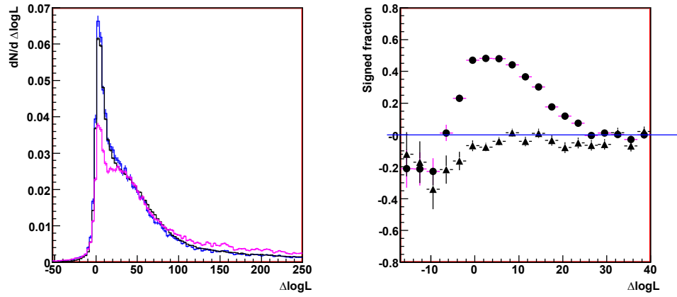
Figure 17: Left: \Delta \log \mathcal{L}_{\pi K} distributions for pions from B^0 \rightarrow \pi^+\pi^- (black) and pions from D^* , before (magenta) and after (blue) reweighting. Right: the relative difference between the D^* and B^0 \rightarrow \pi^+\pi^- \Delta \log \mathcal{L}_{\pi K} distributions before (circles) and after (triangles) reweighting.
