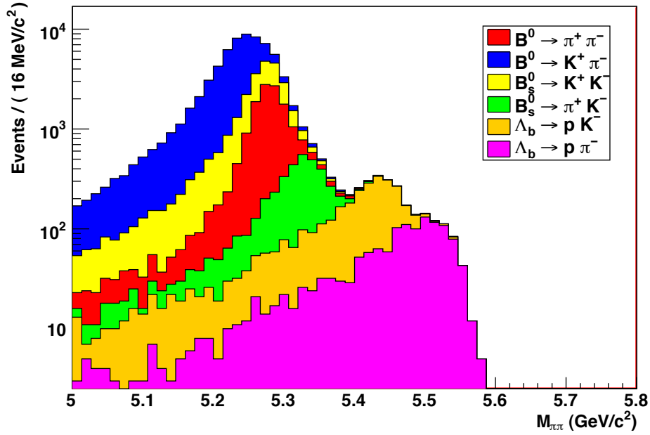
Figure 5: Invariant mass distribution, under the \pi^+\pi^- hypothesis, for all the decay modes after the offline selection: linear scale (top) and logarithmic scale (bottom). The histograms of the various channels are cumulatively added up to form the overall mass line shape. The physical and combinatorial background components are not included.
