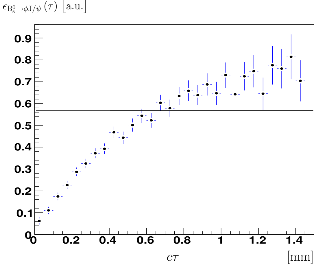
Figure 17: The relative lifetime acceptance function \epsilon_{B_s^0 \rightarrow \phi J/\psi}(\tau) for an applied cut on the direction angle of B_s -meson.
