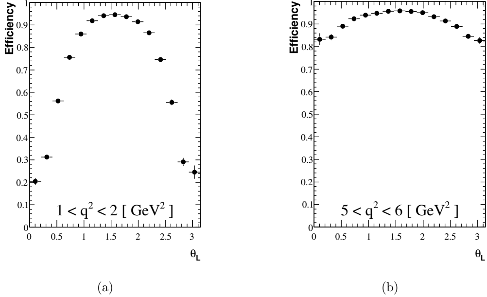
Figure 7: The effect of a 300 MeV \mu p_{\text{T}} cut on the signal efficiency as a function of \theta_{\text{L}} for events with 1 \text{ GeV}^2 < q^2 < 2 \text{ GeV}^2 (a) and 5 \text{ GeV}^2 < q^2 < 6 \text{ GeV}^2 (b).
