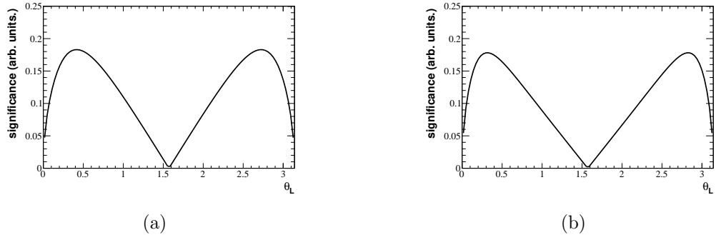
Figure 8: The sensitivity to A_{\text{FB}} as a function of \theta_{\text{L}} for events with 1 \text{ GeV}^2 < q^2 < 2 \text{ GeV}^2 (a) and 5 \text{ GeV}^2 < q^2 < 6 \text{ GeV}^2 (b). The vertical axis shows the statistical significance of a bin in \theta_{\text{L}} for measuring a forward-backward asymmetry with A_{\text{FB}}=0.10 . This is defined as \Delta N_{A_{\text{FB}}}/\sqrt{N} , where \Delta N_{A_{\text{FB}}} is the difference in the number of events expected at a given \theta_{\text{L}} with/without the forward-backward asymmetry, and \sqrt{N} is the statistical uncertainty on the number of events. This is plotted in arbitrary units.
