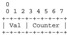
Figure 11: LQL Type 1 Sub-Object Format
