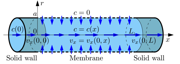
Figure 5 Aldis flow through a cylinder of radius a , of which a section of length L of the wall (dashed) consists of a semipermeable membrane through which a radial flow (small vertical arrows) enters, driven by an osmotic difference in solute concentration c between the internal and external liquids. The axial Poiseuille flow increases (horizontal arrows) for 0 < x < L due to the radial inflow.
