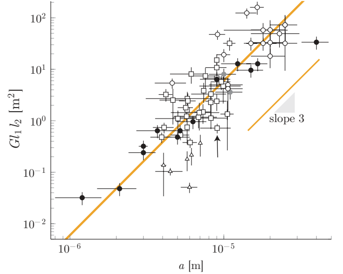
Figure 22 Evidence from field measurements that the radius of phloem sieve elements is optimized for rapid sugar translocation. Comparison between the predicted optimal radius ( a^* ) 3 \sim l_1 l_2 (Eq. (64)) and the measured radius a . Symbols indicate angiosperm herbs (dots), angiosperm trees (open circles), angiosperm shrubs (grey dots), gymnosperm trees (open square), and gymnosperm trees with scales (open triangle). All plants were mature. G is a geometrical factor depending on the cross-sectional shape of the tubes and similarly a is an effective radius. Data from (Jensen et al. , 2011, 2012a)
