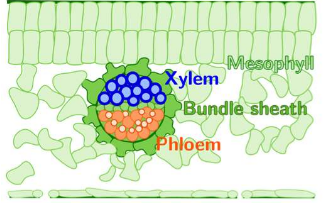
Figure 38 Schematic representation of a cross-section of a leaf. The bundle sheath (dark green) forms a protective layer around the vasculature: xylem tracheary elements (blue) and phloem sieve elements (small circles) with their neighbouring companion cells (orange cells). The water from the xylem passes out through the bundle sheath and presumably along the cell walls of the mesophyll (light green) and most of it evaporates through the stomata (the “holes” in the lower leaf surface). A small part enters the mesophyll where it takes part in the photosynthesis and the subsequent transport of sugars from the mesophyll back in through the bundle sheath, through the companion cells into the sieve elements. Courtesy of Hanna Rademaker.
