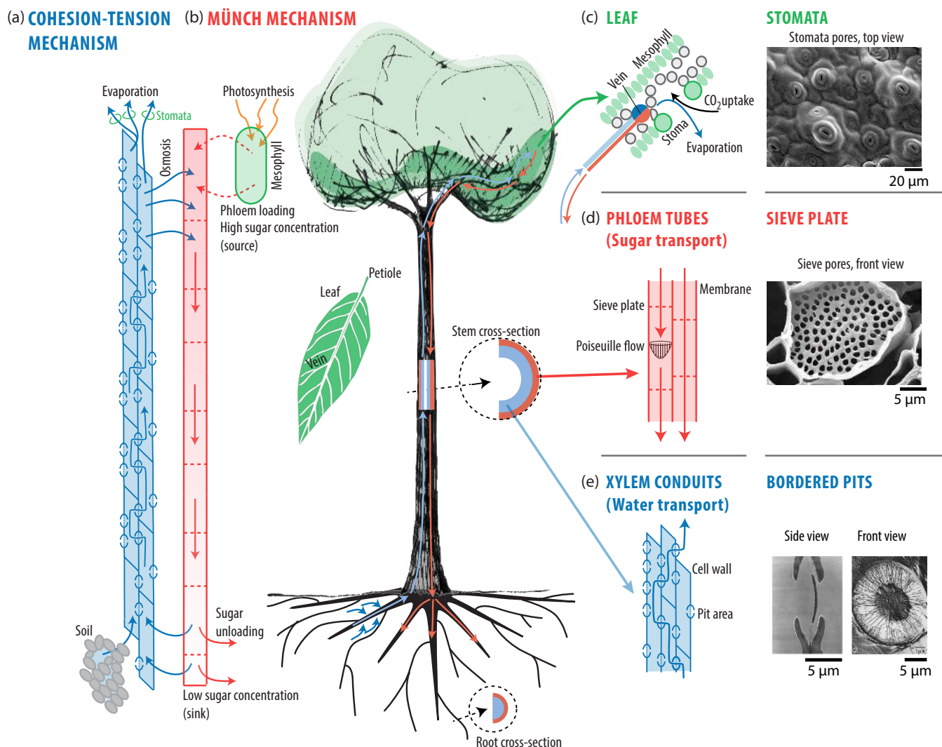
Figure 1 Schematic representation of vascular transport processes in plants. (a) Xylem water transport from soil to shoot is driven by evaporation from leaves via the cohesion-tension mechanism. (b) Phloem sugar transport from leaves to regions of growth is driven by differences in osmotic pressure according to the Münch mechanism. Details of transport processes in (c) leaves, (d) phloem tubes, and (e) xylem conduits are also shown. For clarity xylem and phloem tubes are drawn as same size. See further details in text. (d) As originally published in Jensen et al., Front. Plant Sci. 3, 151 (2012) (Jensen et al., 2012c). (e) Adapted from (Bauch et al., 1972). The background drawing of a tree courtesy of Camille Lucas and Alexandre Ponomarenko.
