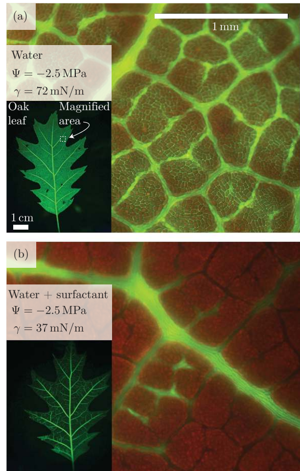
Figure 17 (Color online) Reduction of xylem sap surface tension in oak leaves influences distribution of water in the veins of trees experiencing significant water shortage. Transpiration stream of intact branches on a tree were supplied with either (a) water (surface tension = 72 mN/m) or (b) water mixed with surfactant (0.01% Tween 20, surface tension 37 mN/m). Branches were then cut and allowed to dehydrate to a water potential of -2.5 MPa. At the desired stress level, leaf petioles were cut from the branches while submerged in a fluorescent dye solution (Sulforhodamine G). Leaves infiltrated with water mixed with surfactant experienced significant reduction of dye infiltration to minor veins. Experiments by M. Zwieniecki (unpublished).
