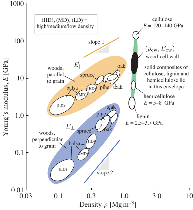
Figure 16 (Color online) Young's modulus E increases with wood density \rho , in rough accord with model Eqns. (38) and (36). Parameters for the pure materials are displayed in the right upper part of the figure, whereas parameters for the composite wood corresponds to the lower density in the yellow (loading parallel to the xylem vessels) and in the blue areas (loading perpendicular to the xylem vessels) of the figure. Adapted from (Gibson, 2012).
