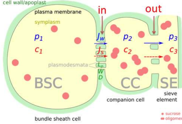
Figure 40 The polymer trap model with diffusion and bulk flow. The bundle sheath cell (BSC) is connected to the companion cell (CC) by narrow plasmodesmata, which prevent the oligomers from diffusing back into the bundle sheath, through the cell interface called “in”. Similarly, the companion cell is connected to the sieve element (SE) through wider plasmodesmata through the “out” interface. The water flow rates J_w through the cell interfaces are marked with blue (full) arrows, the sugar flow rates J_s as red (dashed) arrows. These flows depend on the pressures p as well as on sucrose and oligomer concentrations c_i inside and outside the cells on the loading pathway. The semipermeable cell interfaces are characterized by a permeability L_p , a bulk hindrance factor W , and an effective diffusion coefficient D depending on the structure, density and size of the plasmodesmata connecting them. Adapted from Dölger et al. (2014).
