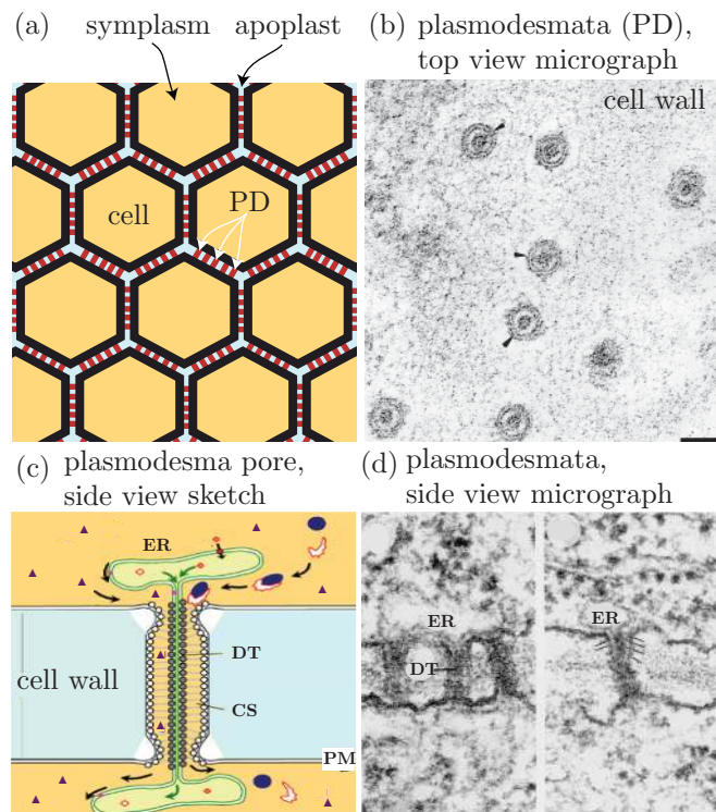
Figure 6 Sketch of plant tissue composed of the living supra-cellular symplasm and the external apoplast. (a) Plant cells (beige) bordered by the plasma membrane (black lines) and connected by narrow plasmodesmata channels (red lines) form the internal living symplasm. They are surrounded by the apoplast (blue) which is the water-filled cell wall matrix. (b) Eight plasmodesmata in the cell wall between two root cells (electron micrograph). (c) Schematic drawing of a plasmodesma pore connecting two cells by forming a channel through the cell wall lined by the plasma membrane (PM). The desmotubule (DT) - enclosed by the endoplasmic reticulum (ER) - fills the center of the pore. The annular space between the plasma membrane and the desmotubule (the cytoplasmic sleeve (CS) marked by arrowheads) allows passage of solutes ( \Delta ) and viral nucleic acids (dark blue ellipsoids). Solutes inside the endoplasmic reticulum might be able to travel from cell to cell through the desmotubule. (d) electron micrographs showing longitudinal views of plasmodesmata. Scale bar = 50 nm. Adapted from (Schulz, 1995):(b,d) and (Schulz, 1999):(c).
