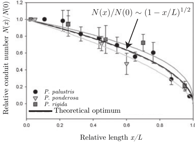
Figure 36 Pine needles are optimized for efficient water transport. Measured axial distribution of number of xylem conduits N(x) plotted as a function of position x along the needle. The base of the needle is located at x = 0 , while x = L corresponds to the tip. Optimum theoretical distribution that minimizes the pressure drop across the needle is plotted as a reference line (Eq. (143)). Adapted from (Zwieniecki et al. , 2006).
