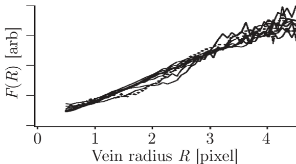
Figure 9 The function F computed from (30) for the seven leaves. As one can see, F(R) is close to linear. Adapted from (Bohn et al. , 2002).
