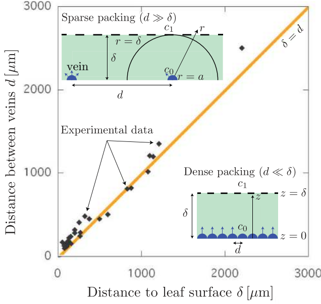
Figure 37 Measured distance between veins d versus distance to evaporative surface \delta for different plant species. The solid line corresponds to the optimal case d = \delta . Adapted from (Noblin et al. , 2008).
