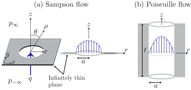
Figure 4 (a) Sampson flow defined as a pressure-driven flow through a circular pore of radius a in an infinitely thin plate. The pressure drop is \Delta p_{\text{smp}} = p_{-\infty} - p_{\infty} , and the flow rate is q . (b) Poiseuille flow along a pore of length t equal to the thickness d of the plate. At low Reynolds numbers, the flow resistance is well approximated by adding the flow resistance from the Sampson and Poiseuille flow, see Eq. (8). Adapted from Jensen et al. (2014) .
