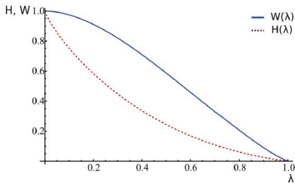
Figure 41 (Color online) Diffusive and convective hindrance factors H (red, dashed) and W (blue, solid) in circular slit pores as function of the relative solute size \lambda . Both approximations given by Dechadilok and Deen (2006) decrease smoothly from 1 to 0 for an increasing solute size, where a hindrance factor of zero corresponds to total blockage of the respective molecule. Above \lambda = 0.8 the curves should be regarded as extrapolations. Adapted from Dölger et al. (2014).
