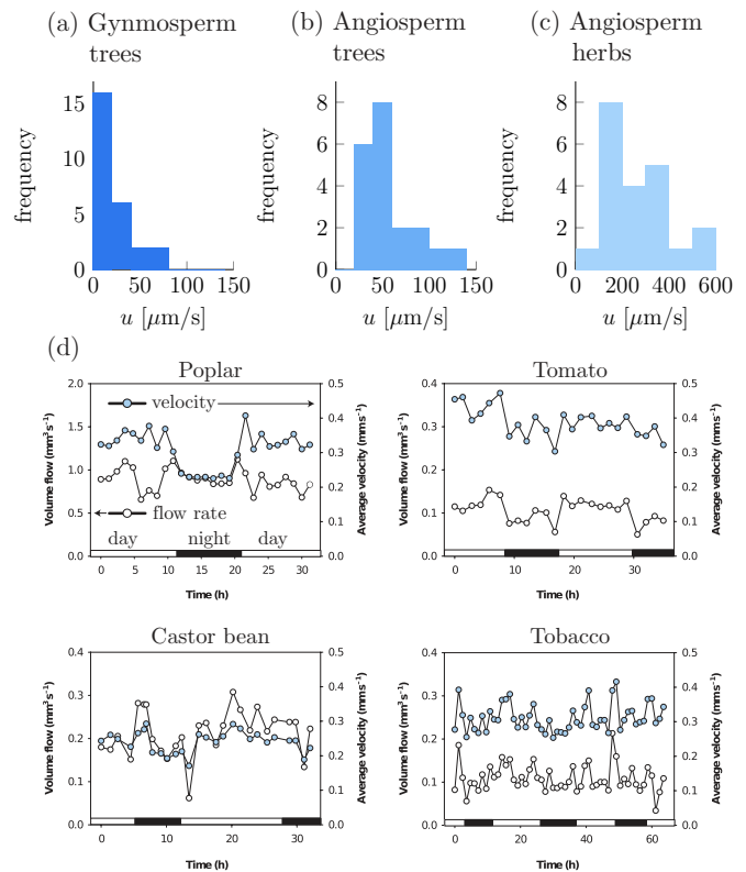
Figure 19 Phloem transport speeds u vary in the range 10^{-5} m/s to 10^{-4} m/s between (a) gymnosperm trees, (b) angiosperm trees, and (c) angiosperm herbs. Panel (d) illustrates the limited diurnal variation in phloem transport rates in four herbaceous angiosperms observed by Windt et al. (2006). Note the difference in abscissa scale between (a,b) and (c). Data from (Liesche et al. , 2015): (a,b) and (Hartt et al. , 1963; Hendrix, 1968; Jensen et al. , 2011; Kursanov, 1956; Moorby et al. , 1963; Mortimer, 1965; Mullendore et al. , 2010; Thompson et al. , 1979; Wardlaw et al. , 1965; Windt et al. , 2006; Ziegler and Vieweg, 1961): (c). Panel (d) adapted from (Windt et al. , 2006).
