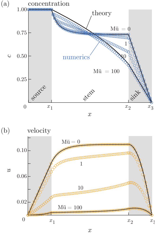
Figure 30 Solutions of the stationary Münch -Horowitz equations for a single tube with “leaf”, “stem” and “root”. Adapted from (Jensen et al. , 2011)
