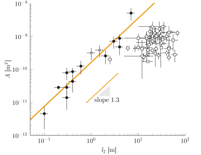
Figure 23 Sieve element cross-sectional area A = \pi a^2 is approximately proportional to stem length l_2 for stems shorter than \sim 10 \text{ m} , and saturates above that height. Symbols indicate angiosperm herbs (dots), angiosperm trees (open circles), angiosperm shrubs (grey dots), gymnosperm trees (open square), and gymnosperm trees with scales (open triangle). Data from (Jensen et al. , 2012b).
