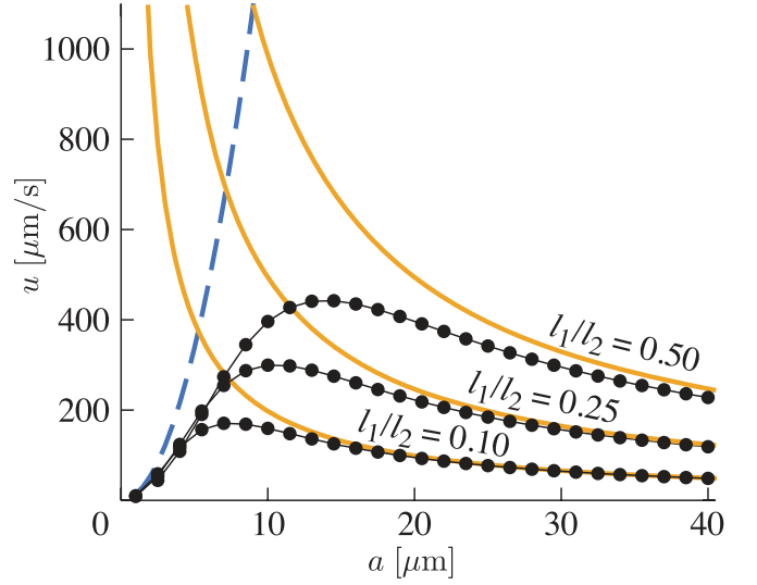
Figure 31 Numerically computed mean velocity \bar{u} as a function of radius a (dots connected by lines) compared to the analytical results for \text{Mü} \ll 1 (Eq. (115), solid lines) and \text{Mü} \gg 1 (Eq. (116), dashed lines). These curves clearly show that \bar{u} grows as a^2 for small a while it decays as 1/a for large a . At the intersection between the two lines given by equation the transition between the two types of flow occurs and the velocity is at a maximum. This is shown also by the dotted curve showing the slightly modified coupled resistor result, Eq. (117). The plots are made with L_p = 5 \times 10^{-14} m(Pa s) ^{-1} , l_1 = (0.1, 0.25, 0.50) m, l_2 = 1 m, RTc_0 = 0.54 MPa, and \eta = 5 \times 10^{-3} Pa s. Adapted from Jensen et al. (2011)
