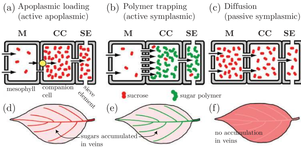
Figure 12 Models of phloem sugar loading strategies according to Turgeon (2010). Represented cell types are sieve element (SE), companion cell (CC), and mesophyll (M). (a) Active apoplasmic loading: sugar transporters (yellow circle) in the companion cell plasma membrane transfers sucrose (red dot) from the apoplast into the sieve element-companion cell complex, energized by a proton pump (not shown). (b) Active symplasmic loading (polymer trapping): Sucrose is transferred from the mesophyll to the companion cell via plasmodesmata gaps in the wall (4 arrows). Here, it is converted under investment of metabolic energy into larger raffinose oligosaccharide family sugar polymers (green dots) that are trapped in the sieve element-companion cell complex. They cannot move back, since the plasmodesmata are too narrow, but can move on into the sieve element through the wide plasmodesma-sieve pore contact. (c) Passive symplasmic loading: sugar diffuses from the mesophyll to the sieve element via plasmodesmata in the companion cell wall. (d), (e) and (f) visualizes the distribution of regions of high sucrose concentration under the the three loading strategies. Accumulation occurs in veins of active apoplasmic loaders and polymer trappers, but not in passive symplasmic loaders. Adapted from (Turgeon, 2010).
