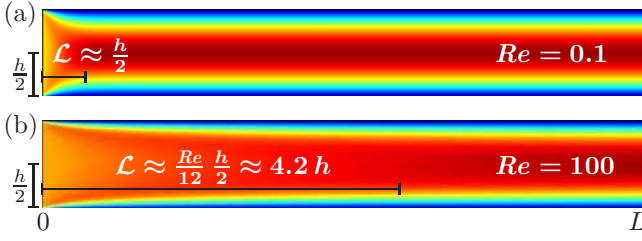
Figure 2 Color plots of the axial velocity from zero (dark blue) to v_x^{\max} (dark red) in a cylindrical channel (side view) of length L and radius a . The velocity field on the inlet to the left is set to be a constant. (a) In the low Reynolds number limit ( Re = 0.1 ) the entrance length over which a full Poiseuille flow profile is established is given by \ell \approx a . (b) In the medium Reynolds number limit ( Re = 100 ) the entrance length is given by Re \approx \frac{Re}{24} a . From Bruus (2011) .
