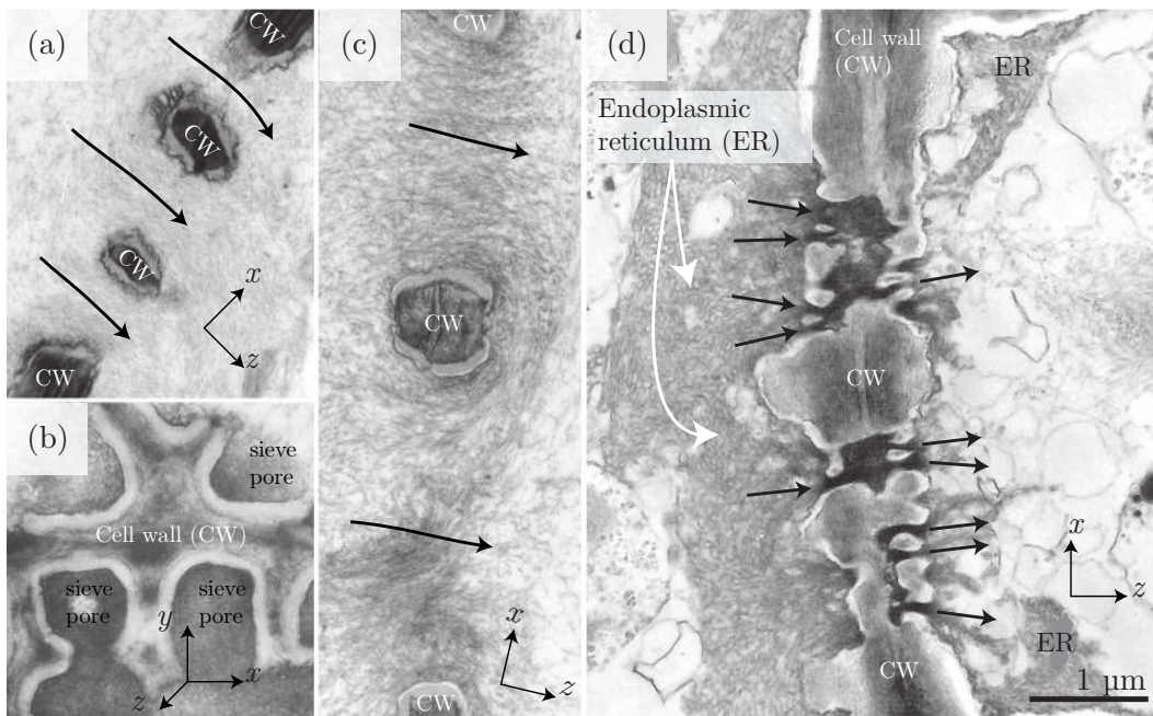
Figure 11 Comparison between phloem sieve plate pores in beech and sieve area pores in spruce, typical for angiosperms and gymnosperms, respectively. (a) Cross section of two sieve pores in a beech sieve plate (see face view of a sieve plate without cellular contents in Fig 1d). Arrows indicate flow paths which are only loosely occupied by hair-like protein filaments (grey). (b) Oblique view of beech sieve pores densely filled with protein filaments. (c) Cross section of sieve pores loosely filled with protein filaments. (d) Cross section of spruce sieve area pores. Arrows mark the orifices of the pores covered on either side with endoplasmic reticulum (ER). The pores form an extended cavity within the cell wall (CW). Scale bar for all panels 1 \mu\text{m} . Adapted from (Schulz and Behnke, 1987).
