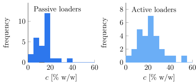
Figure 18 Histograms showing phloem sap concentration measured in plants that utilize passive and active phloem loading strategies (Sec. III.B). See also Fig. 26. Data from Jensen et al. (2013b).
