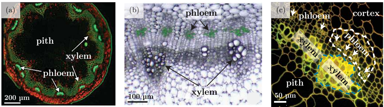
Figure 7 Vascular bundles in the plant stem. (a) Fluorescence micrograph cross section through the stem of Arabidopsis with dull green xylem (X), and bright green phloem (P), translocating water with inorganic ions and sugars, respectively. (b) Bright-field micrograph showing vascular bundles in cauliflower with xylem (X) and phloem (P) overlaid with green fluorescence of sieve elements. (c) Fluorescence micrograph of a young apricot tree stem cross section stained with Coriphosphine O (before the onset of secondary growth). The vascular bundles with phloem (P, white dashed line) and xylem (X, blue dashed line) are embedded in the cortex and pith. Arrows point to the small sieve-element companion cell complexes, responsible for sugar transport. Tracheary xylem elements show strong yellow fluorescence in their lignified cell walls. (a) and (b) adapted from (Khan et al. , 2007). (c) courtesy of Helle J. Martens, Department of Plant and Environmental Sciences, University of Copenhagen
