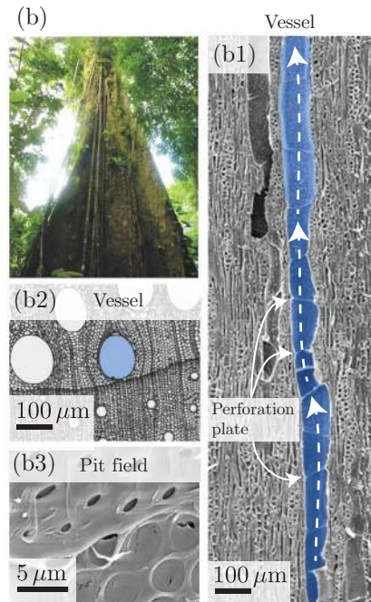
Figure 14 Principles of wood structure in gymnosperms (a) and angiosperms (b). (a1) and (b1) depict typical features of conductive wood (xylem). In gymnosperms, the longitudinal conducting elements (tracheids; (a1), cross section view (a2)) are connected via linearly aligned bordered pits (a3). In angiosperm wood vessels are composed from large cells that are vertically aligned and joined via perforation plates (b1), vessels are also seen as large ovals in cross section (b2). Vessels are connected via fields composed from tens to hundreds of bordered pits (b3). The structure and function of xylem bordered pit pores vary between species (c-e). (c) Bordered pits of gymnosperm with torus and margo, (d) typical angiosperm pit, and (e) angiosperm with vestured pits. Drawings below (c-e) represent cross-sections of bordered pits under normal non embolized conditions, and their potential function as protection from gas spread. (c) From (Core et al. , 1979), (e) courtesy of Steven Jansen, from (Jansen et al. , 2004).
