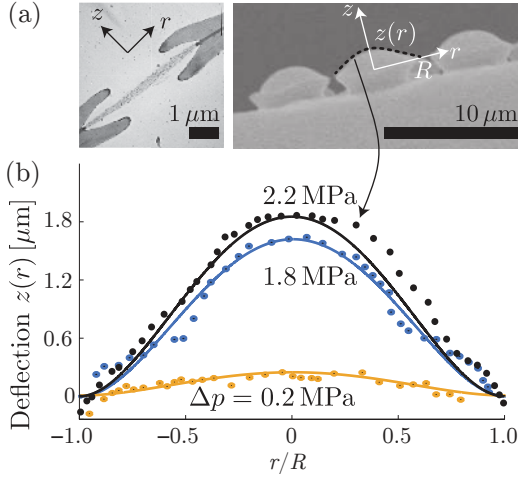
Figure 15 (Color online) Elastic deformation of a pit membrane. (a) Silicone molding of Populus pits at pressure gradient \Delta p = 2.2 MPa. (b) Data points show deflection of the pit membrane as a function of the normalized radial position r/R , measured from molding experiments at pressure gradients indicated in the plot. Solid lines are fits to the linear elastic deflection of a circular plate with clamped edges. Adapted from (Capron et al. , 2014).
