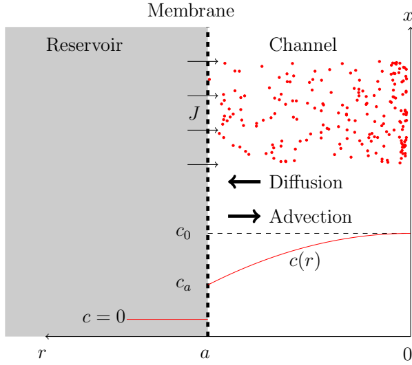
Figure 33 (Color online) Sketch of the solute concentration c(r) [solid red curve and density of dots] in a cylindrical tube of radius a in contact with a reservoir containing pure solvent ( c = 0 ). The semipermeable membrane separating the two solutions is indicated by the thick dashed line. The concentration difference between the reservoir and channel drives an osmotic flow of solvent J \propto c_a across the membrane. This dilutes the solution next to the membrane, and the concentration of solute in contact with the membrane c_a is therefore lower than the value c_0 at the center of the tube. The concentration profile c(r) is set by the relative magnitude of diffusive and advective fluxes (thick arrows). At the membrane interface ( r = a ), there can be no net flux of solute molecules J_s = -D\partial_r c + Jc_a = 0 , which determines the relative magnitude of c_0 and c_a ; see Eq. (136). Adapted from (Haaning et al. , 2013).
