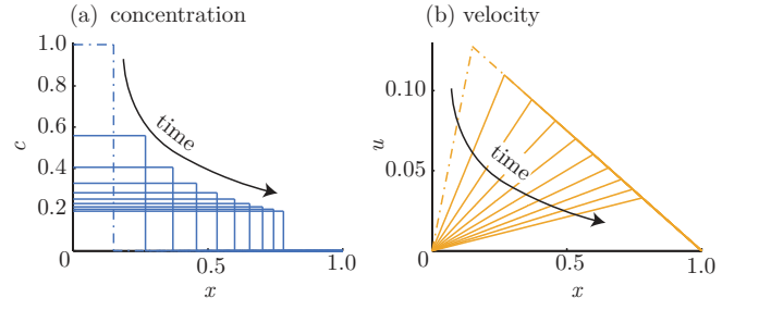
Figure 29 Plot of the analytical solutions (102) for the concentration (a) and for the velocity (b) in a closed, semi-permeable tube with initial sugar concentration given as c_0(x) = c_I = 1 for 0 < x < \lambda = 0.1 and zero elsewhere. The average concentration is \bar{c} = 0.1 . Adapted from Jensen et al. (2009b). Copyright Cambridge University Press. Reprinted with permission.
