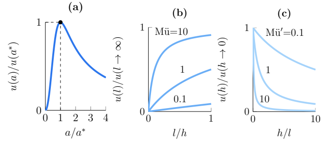
Figure 24 Scaling of the osmotic pumping velocity u (Eq. (69)) with geometric parameters according to Eqns. (70), (71), and (72).
