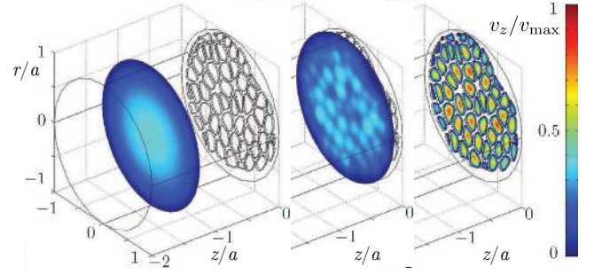
Figure 3 Numerical simulation of the flow moving from left to right close to a Curcubita maxima sieve plate with multiple irregularly shaped pores in a cylindrical pipe. Pore structures were extracted from scanning electron microscopy images ( Mullendore et al., 2010 ). Three color plots of the normalized magnitude v(r, x)/v_{\max} of the flow velocity (from blue zero to red unity) at distances z = 2.5a , 0.25a , and 0.05a from the sieve plate. The flow profile is seen to adapt from the Poiseuille paraboloid to each of the many pores within a distance of a few times a from the sieve plate. As originally published in Jensen et al., Front. Plant Sci. 3, 151 (2012) ( Jensen et al., 2012c ).
