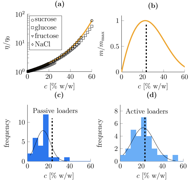
Figure 26 (a) Viscosity increases with concentration by almost two orders of magnitude between c = 0 %wt and c = 60 %wt. Viscosity \eta/\eta_0 plotted as a function of solute concentration c for the substances indicated in the legend. \eta_0 = 1 \text{ mPas} is the viscosity of water and the solid line is a fit to the sucrose data. (b) The mass flux for sucrose (Eq. (75)) is optimal around c = 23 %wt (dashed line). Mass flux m normalized by the maximum value m_{max} plotted as a function of solute concentration c . (c-d) Histograms showing phloem sap concentration measured in plants that utilize passive and active phloem loading. Solid line is a gaussian fit to the frequency distribution. Dashed line shows the optimal concentration, cf. panel (b). Data from Haynes (2012): (a) and Jensen et al. (2013b): (c-d).
