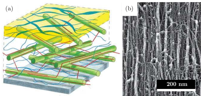
Figure 13 Structure of plant cell walls. (a) Plant cell walls comprise a network of cellulose microfibrils (green rods) linked by hemicellulose (red strands) and pectin (blue strands) to form a network. Lignin confers additional mechanical strength. (b) Electron micrograph of cell wall structure shows mainly cellulose microfibrils after extraction of pectin and hemicellulose. Adapted from (Alberts et al. , 2014)
