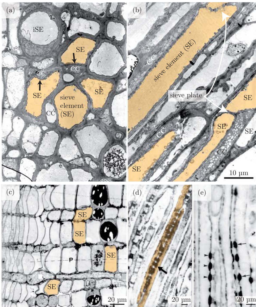
Figure 10 Electron microscopic comparison of the phloem of the flowering plant (angiosperm) beech (a-b) and the non-flowering seed plant (gymnosperm) spruce (c-e). Beige shaded areas are the conducting sieve elements. (a) Transverse cross sections of beech phloem with sieve elements (SE) that are neighbored by companion cells (arrow, CC). The immature sieve element (iSE) still contains a dense cytoplasm. (b) Longitudinal cross section of beech phloem sieve elements (SE) that are neighbored by companion cells (CC) with a dense cytoplasmic content. A sieve plate (SP) separates two adjacent sieve elements. (c) Transverse cross section of spruce phloem (P). Sieve elements appear empty, while parenchyma cells are filled with black tannic acid vacuoles. (d) and (e) Confocal micrographs of live phloem in tangential cross section view, stained with an endoplasmic reticulum specific dye (dark grey). (d) Arrow, end wall of two overlapping sieve elements marked by the many sieve areas, each of them covered on either side by endoplasmic reticulum. (e) Arrows pointing on the sieve areas between two parallel sieve elements. Arrowheads show plasmodesmal connections from a sieve element to a Strasburger cell, which is covered with endoplasmic reticulum on one side only. Adapted from: (a) - (c) (Schulz and Behnke, 1987), (d) (Schulz, 1990), (e) (Schulz, 1992).
