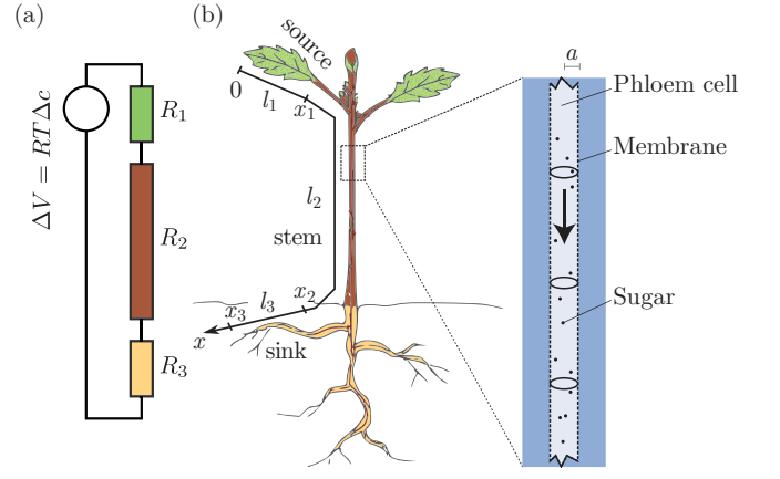
Figure 21 Resistor model of phloem sugar transport. (a) circuit diagram of with resistors representing hydraulic resistance in the source, stem, and sink regions of panel (b). Adapted from ( Jensen et al. , 2011 ).
