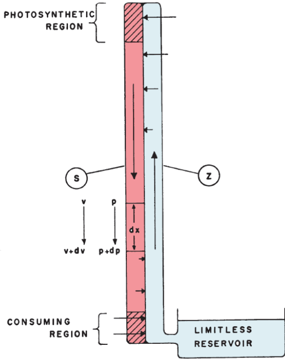
Figure 27 A “1-dimensional tree” according to Horwitz: a tube (S) with semipermeable walls, in contact with another tube (Z) containing pure water, connected to a water reservoir. From Horwitz (1958), reprinted with permission of the American Society of Plant Biologists
