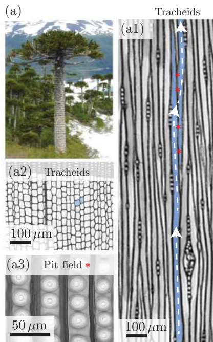
Figure 14 Principles of wood structure in gymnosperms (a) and angiosperms (b). (a1) and (b1) depict typical features of conductive wood (xylem). In gymnosperms, the longitudinal conducting elements (tracheids; (a1), cross section view (a2)) are connected via linearly aligned bordered pits (a3). In angiosperm wood vessels are composed from large cells that are vertically aligned and joined via perforation plates (b1), vessels are also seen as large ovals in cross section (b2). Vessels are connected via fields composed from tens to hundreds of bordered pits (b3). The structure and function of xylem bordered pit pores vary between species (c-e). (c) Bordered pits of gymnosperm with torus and margo, (d) typical angiosperm pit, and (e) angiosperm with vestured pits. Drawings below (c-e) represent cross-sections of bordered pits under normal non embolized conditions, and their potential function as protection from gas spread. (c) From (Core et al. , 1979), (e) courtesy of Steven Jansen, from (Jansen et al. , 2004).
