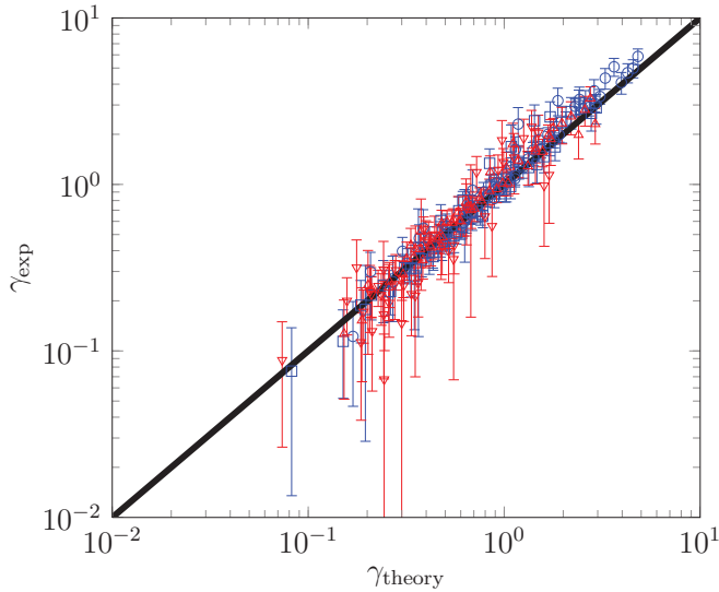
Figure 34 (Color online) Comparison between experimental and theoretical values of the flow rate gain \gamma = u_{out}/u_{in} - 1 obtained using Haaning et al. (2013)’s setup (Fig. 20(e)). Measured values of \gamma plotted as a function of the predicted values using Eq. (137a). Dark blue squares and circles are measurements with NaCl as the solute, for two different lengths of the semi-permeable membrane in the setup, whereas red triangles indicate measurements with sucrose as the solute. Adapted from (Haaning et al. , 2013).
