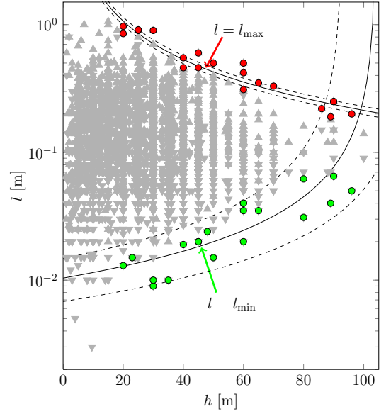
Figure 25 The variability of leaf sizes decreases with plant height, forming upper and lower boundaries (solid lines). Gray triangles show the reported range of leaf sizes for particular species as the longest and shortest leaf lamina length l plotted as a function of tree height h . Solid lines show fits to theory (Eqns. (73) and (74)). Adapted from (Jensen and Zwieniecki, 2013).
