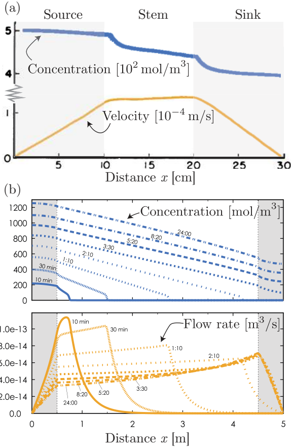
Figure 28 Numerical solutions of the Münch-Horwitz equations by Tyree et al. (1974) and Thompson and Holbrook (2003b) illustrates how the flow velocity increases in the source region, remains approximately constant in the stem, and approaches zero in the sink. The concentration decreases along the plant axis. (a) Shows steady solution by Tyree et al. (1974), while (b) illustrates the flow transient found by Thompson and Holbrook (2003b). Adapted from Thompson and Holbrook (2003b); Tyree et al. (1974). (a) is reprinted with permission of the American Society of Plant Biologists.
