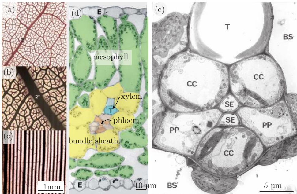
Figure 8 Structure of leaf veins. Venation patterns of (a-b) reticulate and (c) parallel veined leaves. Numbers indicate the vein class. Adapted from (Sack and Scoffoni, 2013). (d) Cross section through a potato leaf at a minor vein. The tissue types are photosynthetically active mesophyll (green) and the bundle sheath (yellow) encircling the vein. The vein has one xylem tracheary element (T, blue), two phloem sieve elements (beige), and three phloem companion cells (beige). (e) Cross section through the smallest vein class (6) of a potato leaf consisting of one tracheary xylem element (T), two phloem sieve elements (SE), three phloem companion cells (CC), and two phloem parenchyma cells (PP). The bundle sheath (BS) surrounds the vein. Adapted from (Schulz et al. , 1998).
