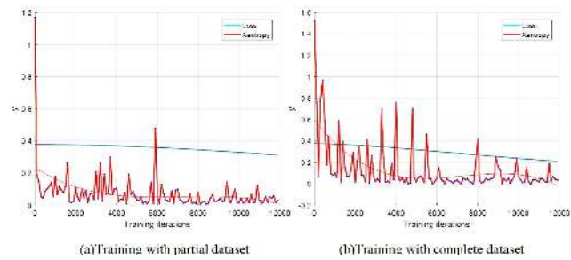
Figure 7. The comparison of training loss and entropy of InspectionNet with (a) partial dataset and (b) the complete dataset.
