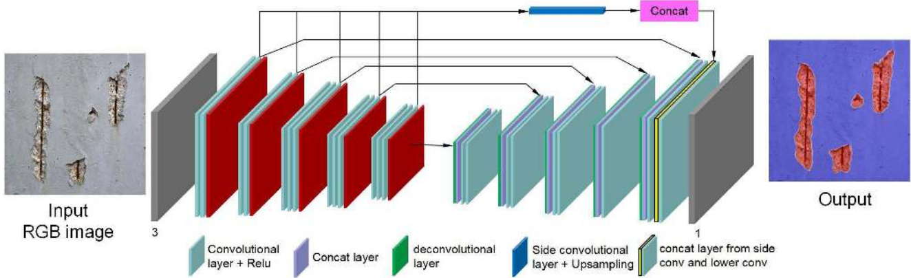
Figure 5. The InspectionNet model, the model has a total 37 layers which is motivated by U-net and HED net.
