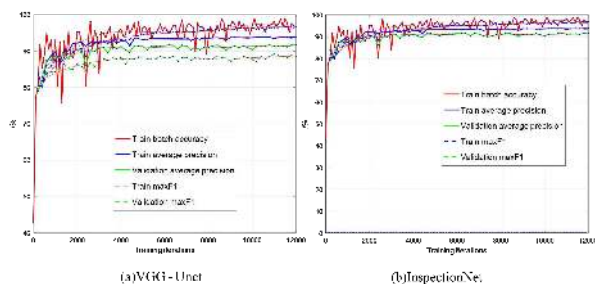
Figure 8. Comparison between (a) VGG-Unet model and (b) our InspectionNet. The perspectives of batch concurrent accuracy, average accuracy and max F1 score are compared.
