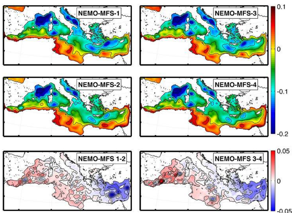
Figure 2. Horizontal maps of the 2-year mean component of the sea surface elevation in the four experiments (units are metres). The two bottom panels represent the sea surface elevation differences between the experiments with and without atmospheric pressure forcing for the time-splitting (right) and the filtered free surface (left) cases.
