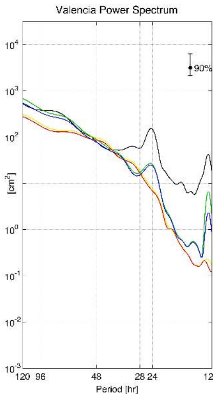
Figure 7. Valencia \eta power spectra from observations and models results. Observations, black; NEMO-MFS1, red; NEMO-MFS2, blue; NEMO-MFS3, yellow; NEMO-MFS4, green.
