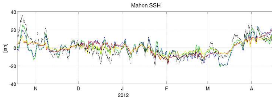
Figure 8. Mahon \eta time-series from observations and model results. Data and model results have been filtered with 5 h running mean. Observations, black; NEMO-MFS1, red; NEMO-MFS2, blue; NEMO-MFS3, yellow; NEMO-MFS4, green.
