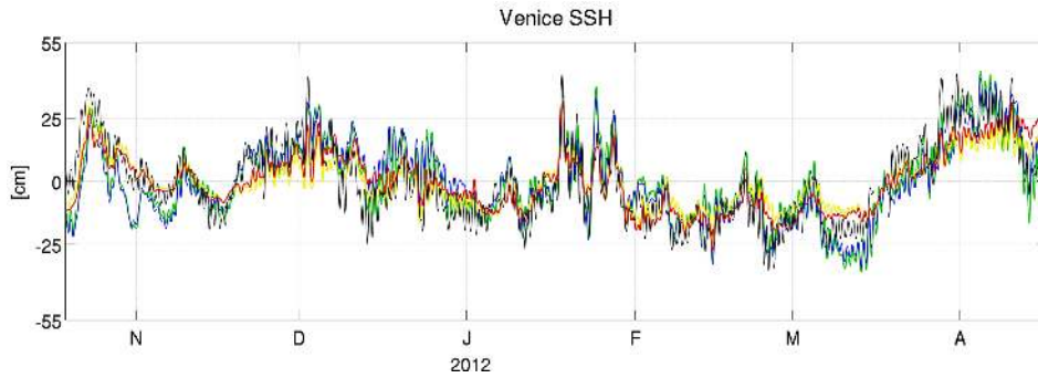
Figure 10. Venice \eta time-series from observations and model results. Data and model results have been filtered with 5 h running mean. Observations, black; NEMO-MFS1, red; NEMO-MFS2, blue; NEMO-MFS3, yellow; NEMO-MFS4, green.
