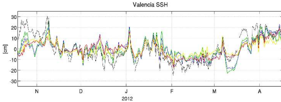
Figure 6. Valencia \eta time-series from observations and model results. Data and model results have been filtered with 5 h running mean. Observations, black; NEMO-MFS1, red; NEMO-MFS2, blue; NEMO-MFS3, yellow; NEMO-MFS4, green.
