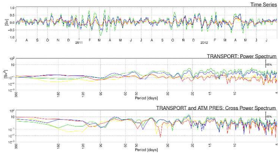
Figure 4. Top panel: Gibraltar transport time-series from the four experiments. Middle panel: Gibraltar transport power spectra. Bottom panel: cross power spectrum between Gibraltar transport and atmospheric pressure. NEMO-MFS1, red; NEMO-MFS2, blue; NEMO-MFS3, yellow; NEMO-MFS4, green.
